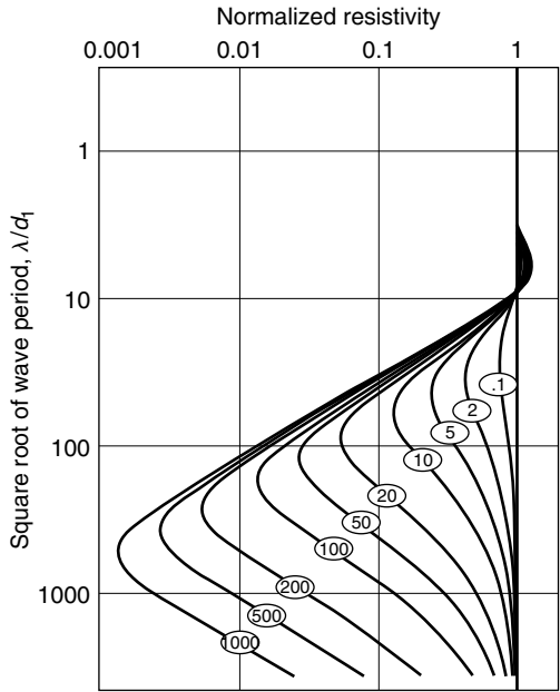
Figure 13.12 Magnetotelluric sounding curves for a three-layer sequence. The middle layer is more conductive than the first and last layers, which both have the same resistivity. The resistivity of the middle layer is indicated by the label on each curve.
