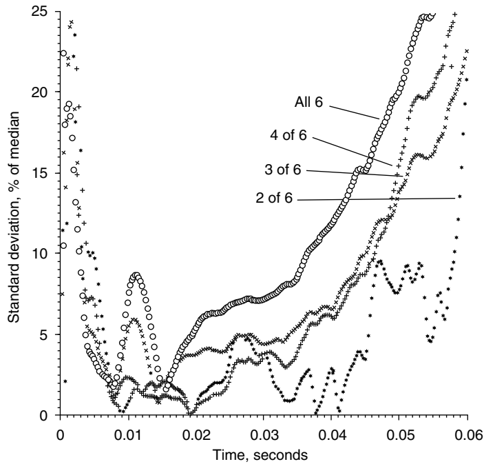
Figure 11.30 Standard deviation characterizing the scatter of points when several signals are stacked. These curves show the scatter on stacking 2, 3, 4, or all 6 of six signals. Selection of the signals to be stacked was based on similitude between signals.
