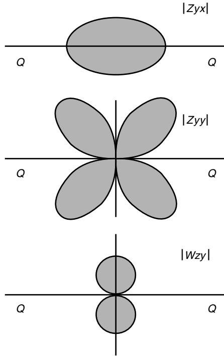
Figure 13.20 Typical forms of polar diagrams for MT soundings over a two-dimensional geoelectric structure.
