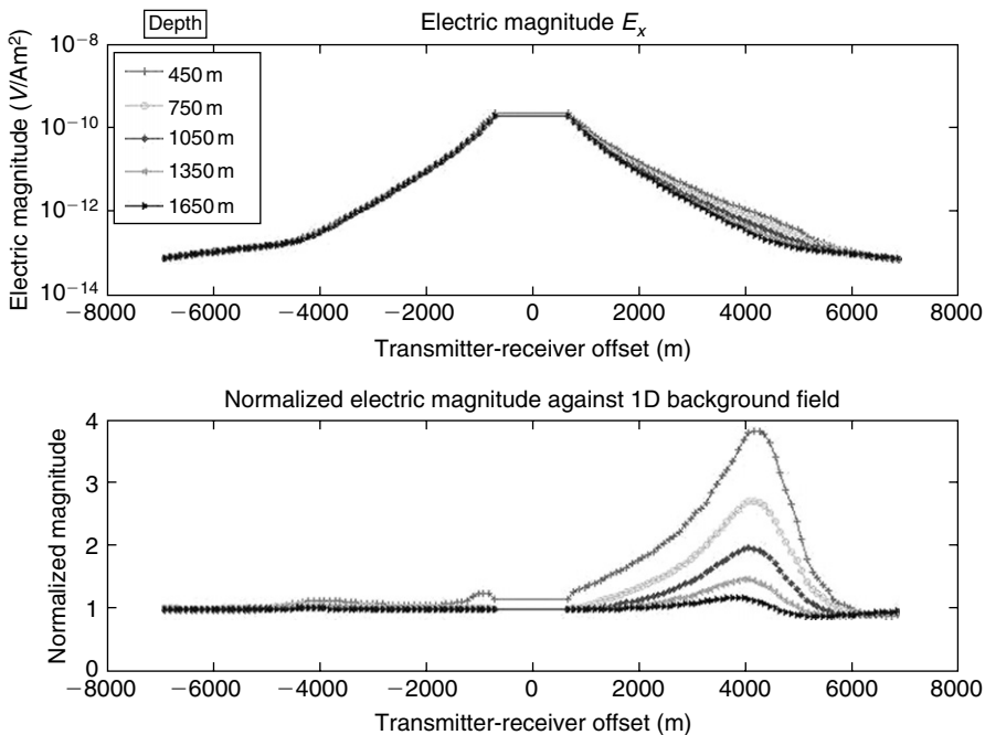
Figure 15.14 Plots of the electric field magnitude versus offset for a model with the resistive reservoir located at different depths.
