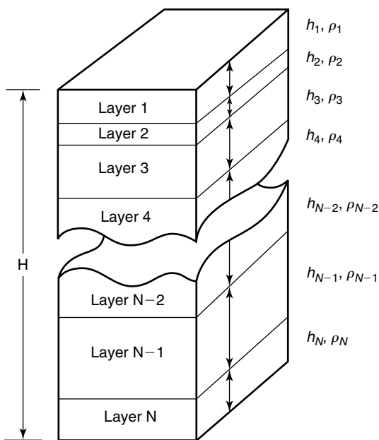
Figure 10.22 Column of rock one meter square hypothetically cut from a layered sequence of rocks. This column is used to define average longitudinal resistivity, average transverse resistivity, and anisotropy.
