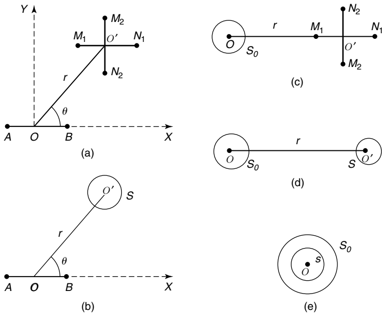
Figure 14.1 Plan view of commonly used transmitter-receiver pairs. When small loops are used as magnetic dipoles, either transmitting or receiving, their orientation is best described in terms of the direction of their moment, which is normal to the plane of the coil.
