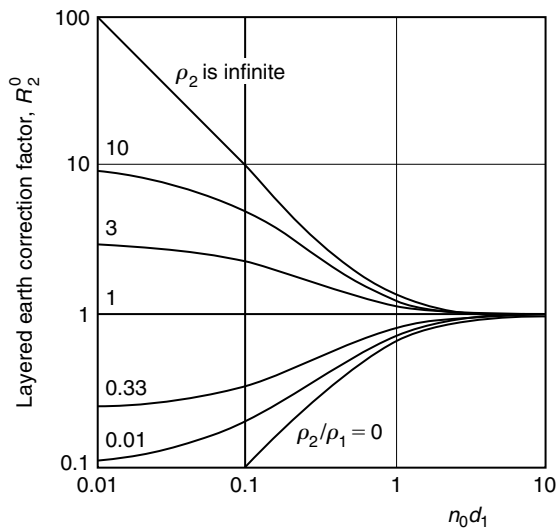
Figure 5.4 Layered-earth correction factor at DC for a sequence of two layers (an overburden and a lower half-space) as a function of the contrast in resistivity between two layers.
