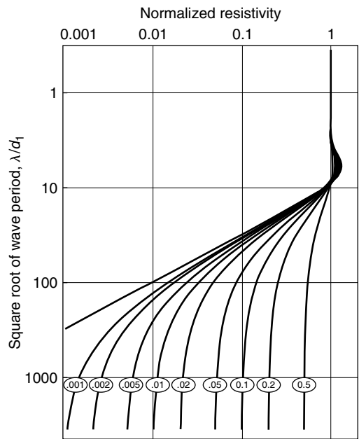
Figure 13.9 Magnetotelluric sounding curves for a two-layer sequence in which the second layer is more conductive than the first. The contrast between the resistivity of the second layer and the resistivity of the first is indicated by the label on each curve.
