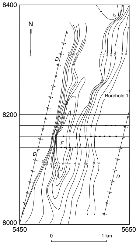
Figure 16.12 Results of a mise-a-la-masse survey in the Miihkali area of Finland. The current electrode A is placed in a conductive orebody intersection at a depth of 730 meters in Borehole 1. The values contoured are voltages measured over the surface divided by the current flowing to electrode A.
