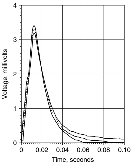
Figure 11.31 Results of stacking three signals with best similitude.
