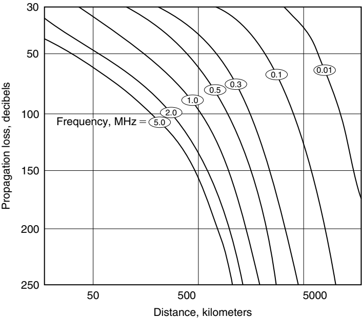
Figure 16.5 Propagation loss for electromagnetic surface waves traveling over a smooth spherical earth. Assumed conductivity of 0.005 S/m and relative dielectric constant of 15. Energy is radiated from a short vertical antenna. Power radiated is 1 kilowatt which produces a field strength of 300 millivolts per meter at 1 kilometer from the antenna.
