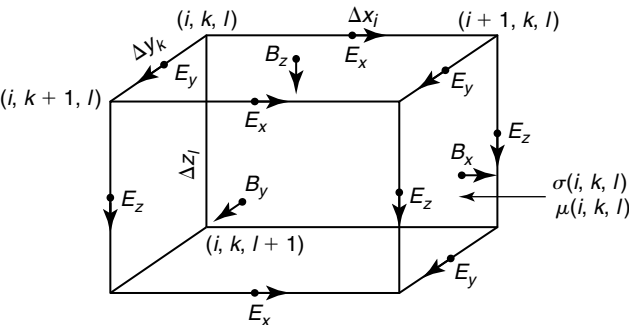
Figure 6.5 Discretization of the electromagnetic field on a staggered grid, according to Yee (1966) and Wang and Hohman (1993). The electric field components, parallel to the corresponding edges, are sampled at the centers of the prism edges, while the magnetic field components, orthogonal to corresponding faces, are sampled at the centers of the prism faces.
