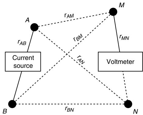
Figure 12.1 Plan view of a generic four-electrode array for measuring earth resistivity. The four electrodes can be arrayed quite arbitrarily, and yet an apparent resistivity value can be computed knowing only the electrode distances, the current, and the voltage.
