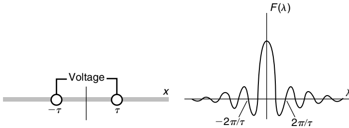
Figure 11.13 Filtering phenomenon which occurs when an electric field is measured with electrodes at a nonzero separation (on the left). The actual electric field can vary markedly between the two electrodes, with the measured voltage representing the average electric field between the electrodes. The system response of this system is shown in the space frequency domain on the right.
