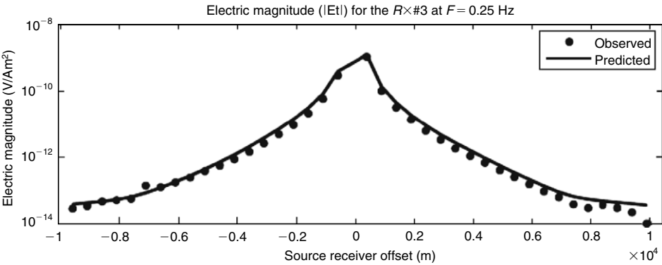
Figure 15.30 Amplitude versus offset (AVO) plots of the Troll Field data at a frequency 0.25 Hz. The black dots show the observed in-line electric field data, while the predicted data for a model obtained by iterative migration are plotted by a solid line.
