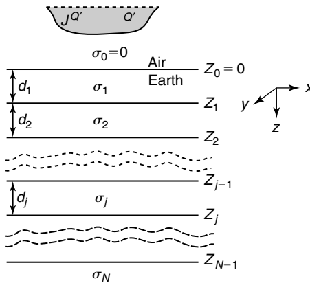
Figure 13.16 Model used in discussion of a magnetotelluric sounding of a layered earth. The source of the field is assumed to be a current system circulating at high altitude. The downward traveling electromagnetic field excites current flow in conductive layers in the earth. The electric field induced in the earth and the secondary magnetic field accompanying currents in the earth are the quantities to be measured in carrying out a magnetotelluric sounding.
