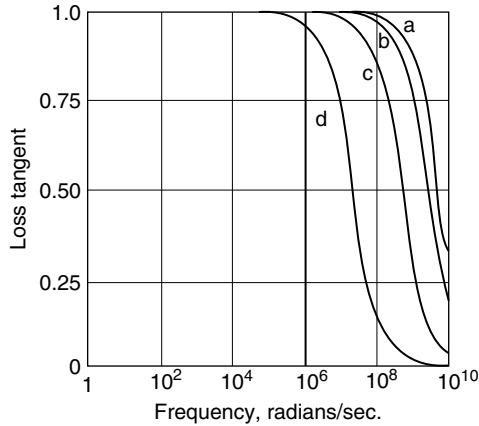
Figure 16.9 Loss tangent for electromagnetic waves propagating through a uniform conductive medium. Four cases are shown: a) seawater, conductivity = 4.0 S/m, dielectric constant = 82.4; b) soft shale, conductivity = 0.5 S/m, dielectric constant = 20; c) sandstone, conductivity = .05 S/m, dielectric constant = 10; and d) granite, conductivity = .001 S/m, dielectric constant = 4.85.
