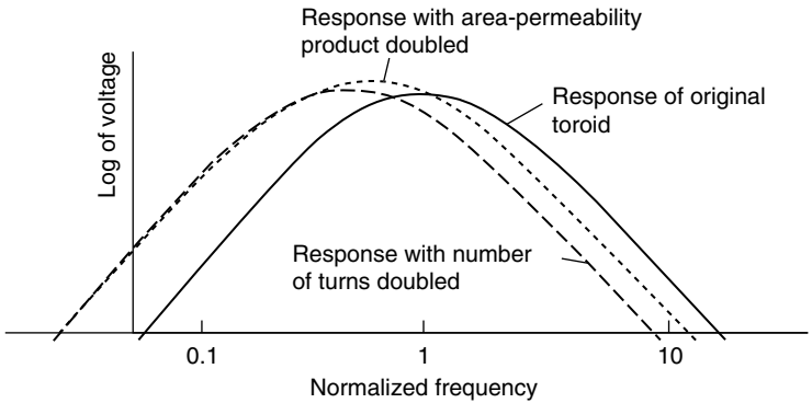
Figure 11.21 Changing the response of an induction coil. Increasing the number of turns will provide more output at lower frequencies but lower output at high frequencies. Increasing the area-permeability product of the coil will cause a somewhat similar change in output.
