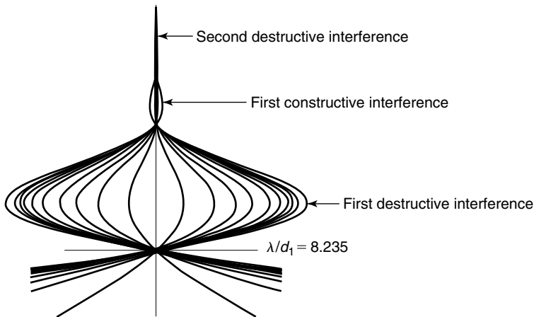
Figure 13.11 Detail of the magnetotelluric sounding curves in the neighborhood of the first crossing of the unit axis.
