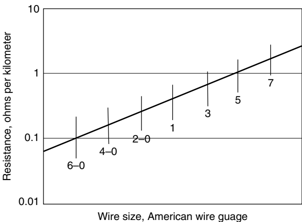
Figure 11.5 Resistance of stranded copper wire at 20°C.
