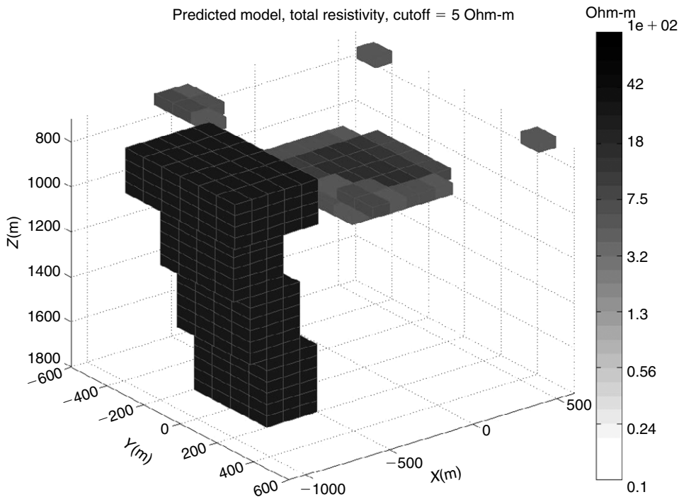
Figure 15.26 Model 2. 3-D image of the result of the inversion of the data contaminated by random noise. The true salt dome background conductivity model is used in the inversion.
