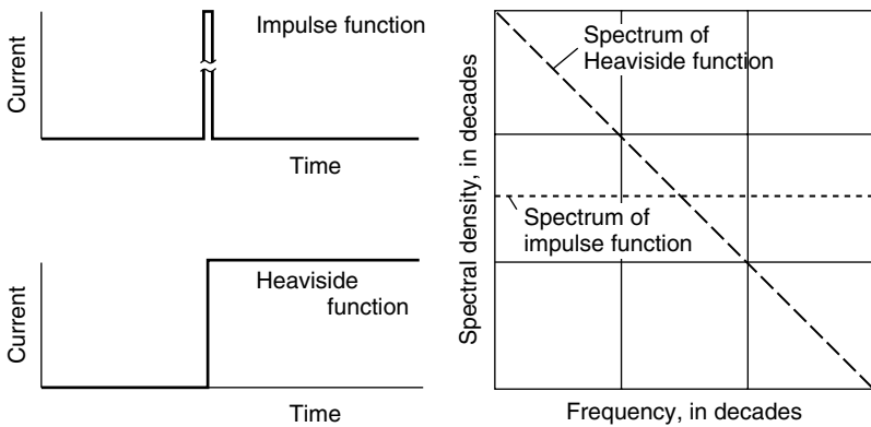
Figure 5.9 Two wave forms commonly used for time-domain electromagnetic soundings. The impulse wave form is of short duration but great amplitude. Ideally, for zero width and infinite amplitude, the spectrum of an impulse is constant at all frequencies. The Heaviside function is the time integral of an impulse. The spectrum of a Heaviside function declines in amplitude linearly as frequency increases.
