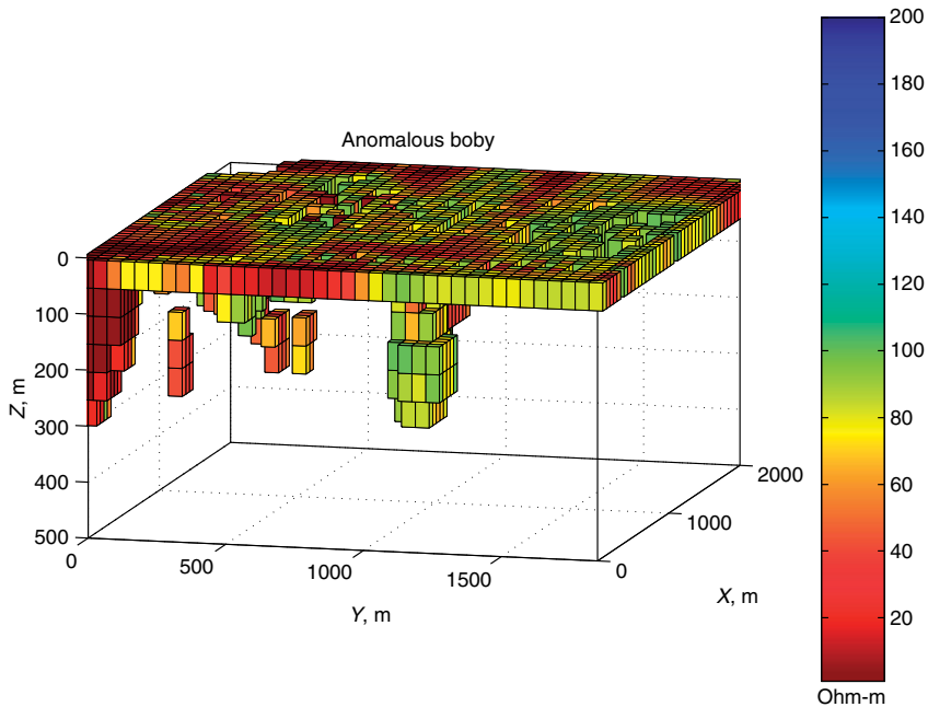
Figure 13.33 Volume image of the result of the MT data inversion in Deerlock Property.
