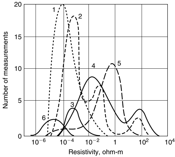
Figure 10.4 Histograms for the reported values of the resistivity for common minerals with high conductivity: 1) Bornite; 2) Magnetite; 3) Pyrrhotite; 4) Arsenopyrite; 5) Galena; 6) Covillite.
