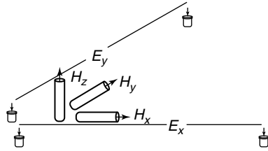
Figure 13.18 Layout of sensors for a single magnetotelluric sounding. Three components of the magnetic field are measured, using sensitive vector magnetometers, often induction coils. Two components of the electric field are detected by measuring the voltage between pairs of electrodes, usually separated by a distance of a few hundred meters.
