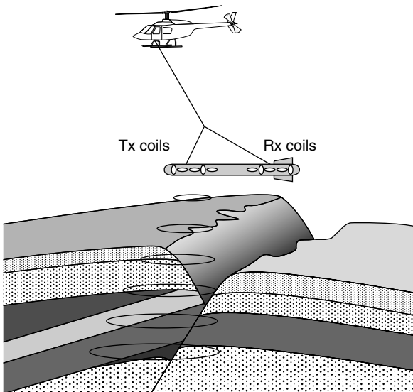
Figure 16.2 A typical airborne EM system has several transmitter-receiver pairs. For example, the DIGHEM system has five transmitter-receiver pairs, three of which form a coplanar array with the transmitter and receiver coils transmitting/measuring only the vertical components of the EM field, and two coils forming a co-axial array with the transmitter and receiver coils transmitting/measuring only the horizontal components of the field.
