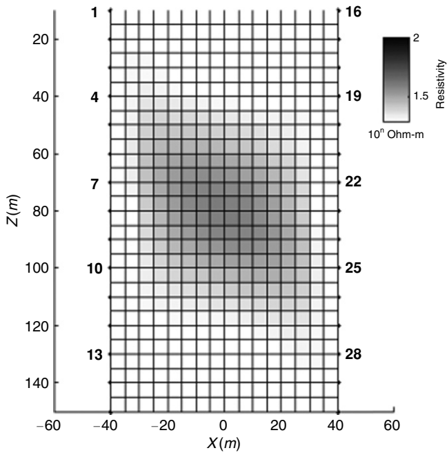
Figure 16.16 A vertical slice through two boreholes of the model obtained as a result of smooth inversion of the crosshole tomographic data.
