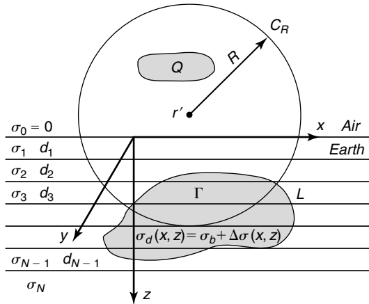
Figure 6.2 The two-dimensional model of a localized cylindrical inhomogeneity \Gamma with the conductivity \tilde{\sigma}(x, z) = \tilde{\sigma}_b + \Delta\tilde{\sigma}(x, z) embedded in a background (normal) horizontally stratified section characterized by a conductivity sequence, \tilde{\sigma}_b(\tilde{\sigma}_1, \tilde{\sigma}_2, \dots, \tilde{\sigma}_n) . The structure is illuminated with an E -polarized field, which originates from linear currents distributed with the density \mathbf{j}^e = j^e \mathbf{d}_y flowing in a region Q in the upper half-space.
