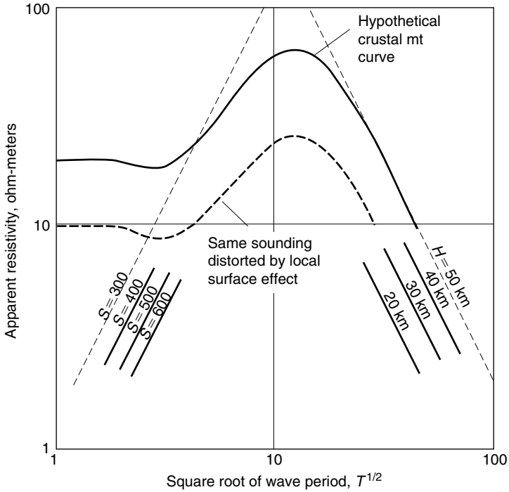
Figure 13.22 Static shift of a magnetotelluric curve occurs when the electric field measurement is distorted proportionately more than the magnetic field by a small-scale inhomogeneity in the conductivity of the rock in which the electrodes to measure the electric field are sited. Static shift usually causes an overestimate of the conductance of the surface layer and an underestimate of the depth to the conductive part of the crust.
