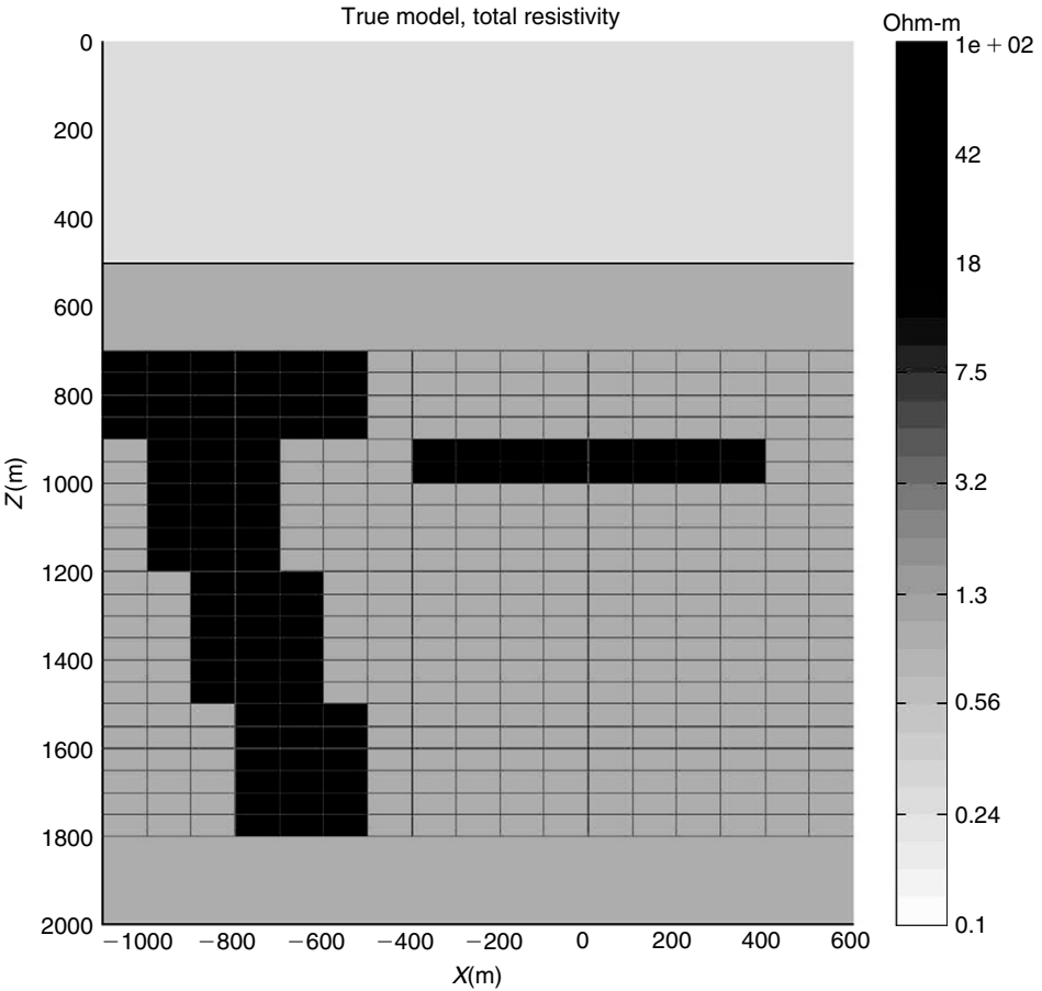
Figure 15.23 Model 2: a petroleum reservoir in the presence of a salt dome structure (vertical section). The area shown with grids defines the extent of the anomalous domain in the inversions.
