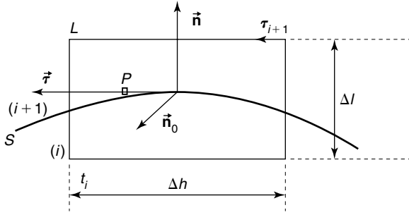
Figure 3.4 The behavior of the tangential components of the electromagnetic field in the transitional layer with a thickness \Delta\ell in which the parameters \epsilon , \mu , and \sigma vary rapidly but continuously.
