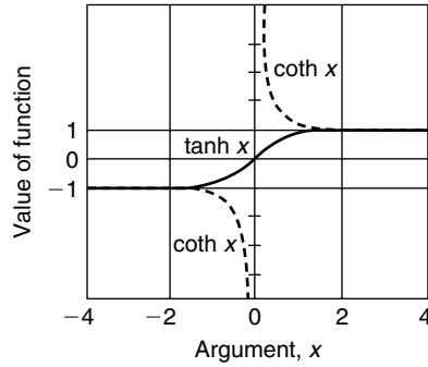
Figure 5.3 Values for the hyperbolic tangent and cotangent. Note that the values for tangent lie between -1 and 1, while the values for the cotangent lie only outside this range.
