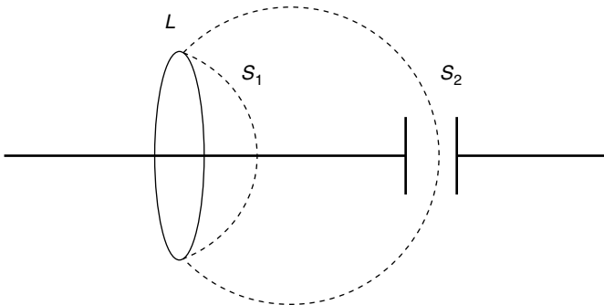
Figure 3.2 Illustration of the concept of displacement currents introduced by Maxwell.
