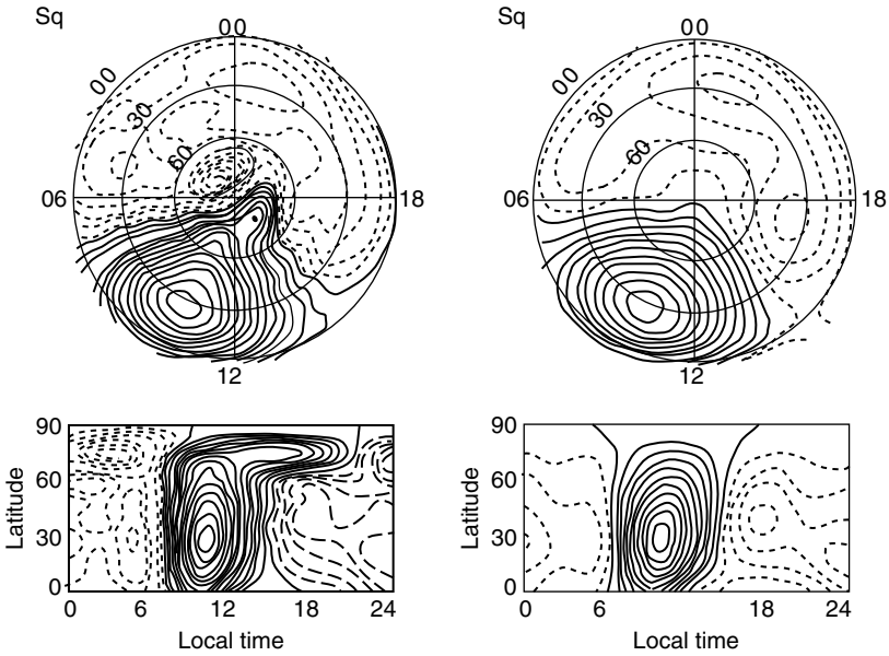
Figure 13.2 Ionospheric current pattern used to explain the observed changes in magnetic field on a quiet day. The right-hand panels include only tide-produced currents, while the panels on the left include convecting polar currents as well. The current between adjacent paths is 10,000 amperes in a counterclockwise direction for solid lines, and 10,000 amperes in a clockwise direction for dashed lines.
