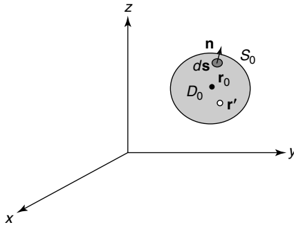
Figure 2.1 The volume density of the sources of the vector field \mathbf{B} is calculated as a limit of the integral over volume D_0 , bounded by a closed surface S_0 , of the divergence of the vector field divided by the volume D_0 when the volume tends to zero: D_0 \rightarrow 0 .
