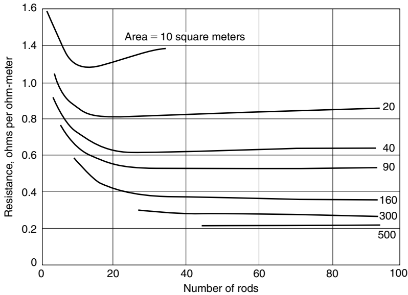
Figure 11.8 The minimum resistance obtainable by driving a given number of rods in a given area.
