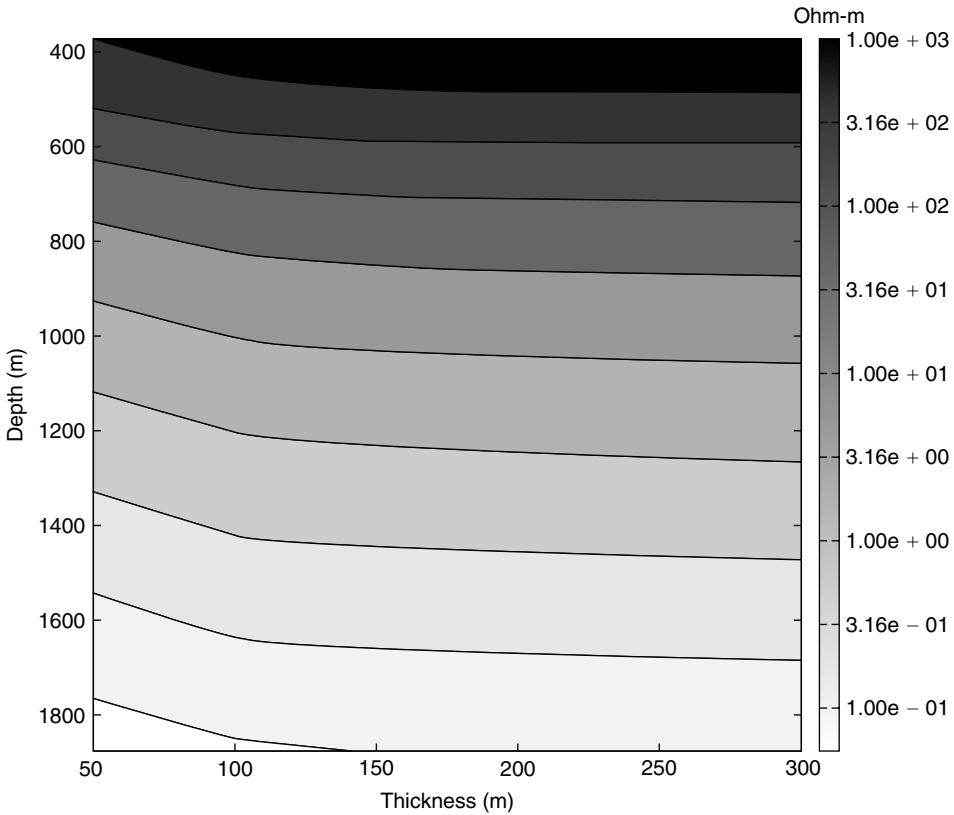
Figure 15.16 The integrated sensitivity for different thicknesses and depths of the resistive body.
