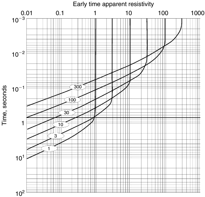
Figure 14.8 Apparent resistivity curves computed with the early-time asymptotic expression for a uniform earth. The separation from transmitter to receiver is 1000 meters. The resistivity of the earth is shown by the label on each curve.
