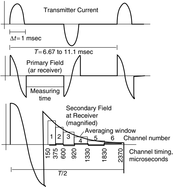
Figure 16.4 Description of the operation of the ATEM airborne electromagnetic system. A transmitter coil is energized with separated half-sinusoidal current pulses. These generate a primary field in the form of half-cosinusoids at a receiver coil towed behind the aircraft. The secondary signal caused by induction in the earth is a transient waveform which appears during the transmitter-off period. This secondary signal is sampled over six boxcars, as indicated.
