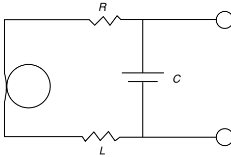
Figure 11.19 Representation of an induction coil as an equivalent circuit with lumped resistance, capacitance, and inductance.
