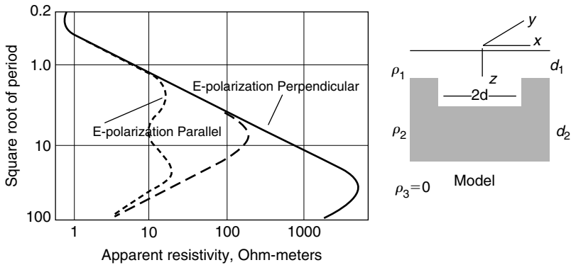
Figure 13.25 Distortion caused to magnetotelluric sounding curves by lateral changes in the geoelectric structure. The model is that of a graben extending in the y -direction. The solid curve and the short-dashed curve were computed for electric-field polarizations as indicated. The long-dashed curve is the curve corresponding to a one-dimensional model in which the surface layer has the thickness corresponding to the depth of the graben.
