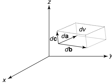
Figure 1.6 An infinitesimally small element of volume dv is represented as a parallelepiped formed by three vectors, d\mathbf{a} , d\mathbf{b} , and d\mathbf{c} .
