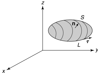
Figure 1.4 Formulation of Stokes's theorem. The direction of the positive normal to the surface S depends on the choice of the positive direction along the contour L . A standard convention is that, traversing of the contour in the positive direction \boldsymbol{\tau} can be treated as a clockwise movement for the observer looking in the direction of the positive normal \mathbf{n} .
