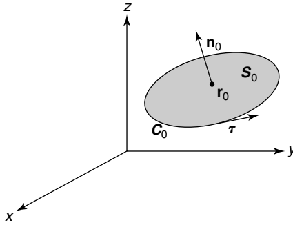
Figure 2.2 The volume density of the vortices of the vector field \mathbf{B} is calculated as a limit of a scalar flux of the curl of the vector field over surface S_0 , bounded by a closed contour C_0 , divided by the area S_0 when the area tends to zero: S_0 \rightarrow 0 .
