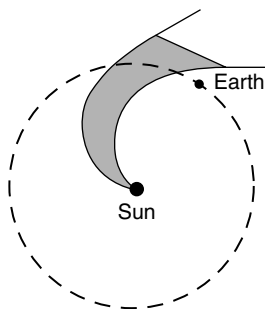
Figure 13.1 Apparent path of a jet of solar plasma from the Sun to the earth.
