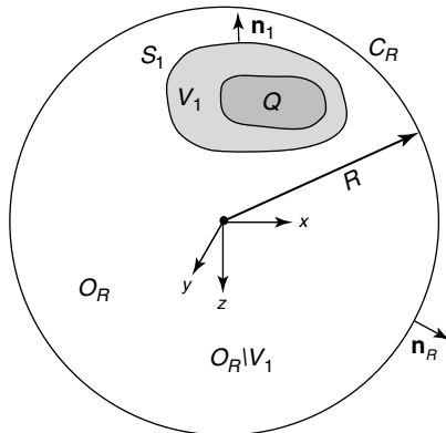
Figure 3.5 Derivation of Poynting's theorem, the energy inequality, and Lorentz lemma.
