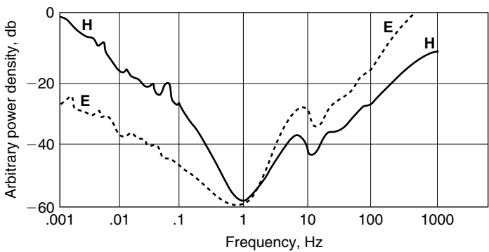
Figure 13.4 Typical power density spectra for the time varying electric and magnetic fields of the Earth. The strength and the detailed structure will vary with time and place.
