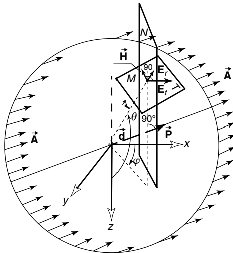
Figure 4.8 Geometrical representation of a spherical electromagnetic wave.
