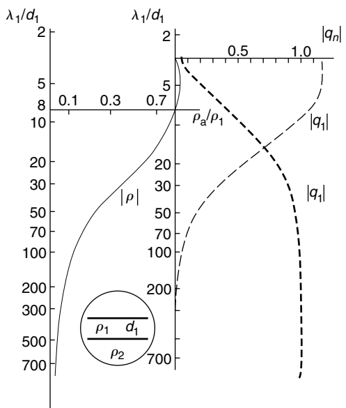
Figure 13.6 Construction of an MT curve for two layers, the lower one having 1/9 the resistivity of the upper one, by summation of the contribution from each of the two layers.
