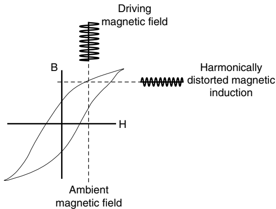
Figure 11.16 Principle of the flux-gate magnetometer. The sensing element is a ring or rod of ferromagnetic material with a hysteresis curve as shown. An oscillatory magnetic field (1-100 kHz) is added to the ambient magnetic field by driving a monochromatic current through a coil wound on the sensing element. Because the hysteresis curve is curved, the magnetic induction exhibits harmonic distortion. The second harmonic is separated by filtering and used to determine the strength of the ambient field.
