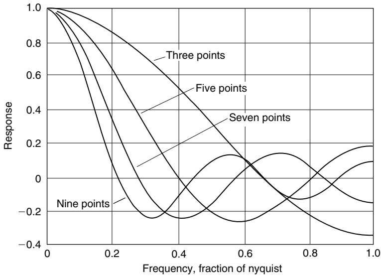
Figure 11.25 Frequency response of running average (boxcar) filters.
