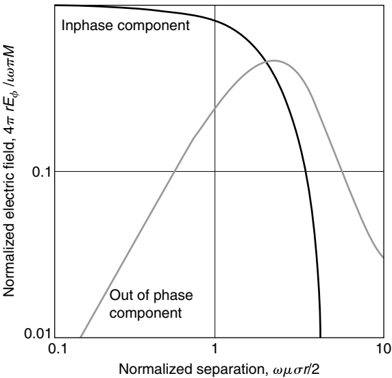
Figure 14.3 Tangential electric field on the surface of a uniform earth generated by a vertical-axis magnetic dipole source. The plots show the absolute values of the real and imaginary parts of the normalized mutual impedance in logarithmic scale. Note that according to the principle of reciprocity, these same curves apply to the case of a current dipole source and detection of the vertical component of magnetic induction.
