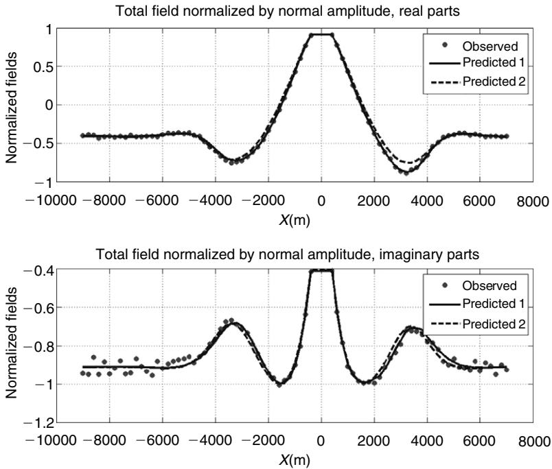
Figure 15.19 Model 1. Plots of the real (top panel) and imaginary (bottom panel) parts of the normalized observed and predicted in-line electric fields E_x at a frequency of 0.75 Hz for receiver #3 ( x = -6,000 m, y = 0 m). The dots show the noisy observed data, while the predicted data for a model obtained by the inversion are plotted by the lines. The solid line corresponds to the predicted data (“predicted 1”) obtained by inversion with the true 1-D background model, while the dashed line shows the predicted data (“predicted 2”) computed for 3-D inversion result obtained with the background model found by 1-D inversion.
