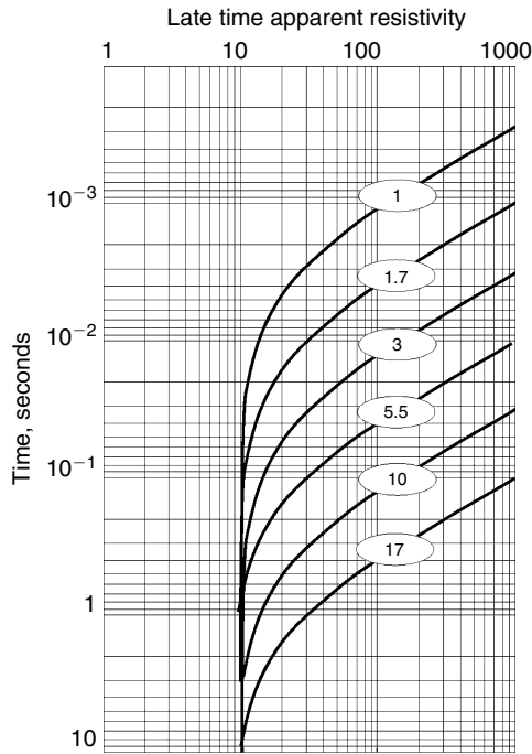
Figure 14.7 Time-domain electromagnetic sounding curves for a uniform earth with a resistivity of 10 ohm-meters. The source-receiver separation (in kilometers) is indicated by the label on each curve.
