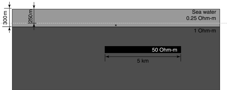
Figure 15.13 Model of a resistive rectangular target (petroleum reservoir) located within a conductive sea-bottom formation.
