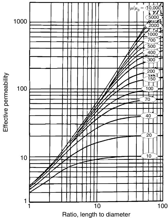
Figure 11.20 Effective permeability of a cylindrical rod of high-permeability material.
