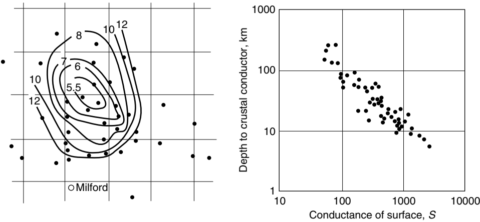
Figure 13.23 Example of the generation of a false crustal structure by static shift. An MT survey was carried out in central Utah near the town of Milford as shown on the map at the left. Depth to a postulated crustal conductor was estimated from the descending asymptote of the observed magnetotelluric sounding curves, with the depths shown as contoured. The plot on the right shows the correlation between the conductance of the near-surface layer, as estimated by the rising asymptote of the MT curves, and the estimated depth to the crustal conductor. The close inverse correlation between these two quantities is strong evidence for the feature being generated by static shift of the MT curves. (The grid on the map at the left has a ten kilometer grid superimposed).
