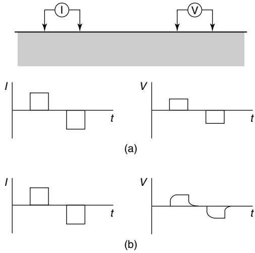
Figure 12.8 Sketch of the potential waveform for a current injected into nonpolarizable and polarizable ground. Panel (a) shows the case of non-polarizable ground and (b) shows that of polarizable ground.
