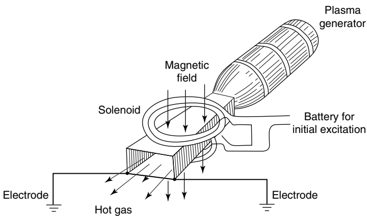
Figure 11.1 Elements of an uncooled magneto-hydrodynamic generator. A hot ionized gas is created in the plasma generator. This gas flows through a channel under the action of a magnetic field. The ions are directed and collected to form an output current which is then fed to the ground through electrodes.
