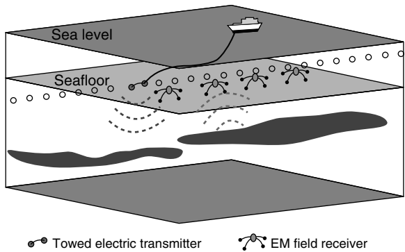
Figure 15.12 General survey configuration of the MCSEM method. An electric bipole transmitter towed by the survey vessel generates an EM signal, while the fixed multi-component EM field receivers located on the seafloor measure the EM response from the geoelectrical structure beneath the seafloor.
