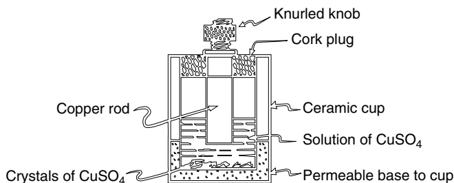
Figure 11.11 Construction of a porous pot salt bridge for use in detecting voltage in a material with electrolytic conduction.
