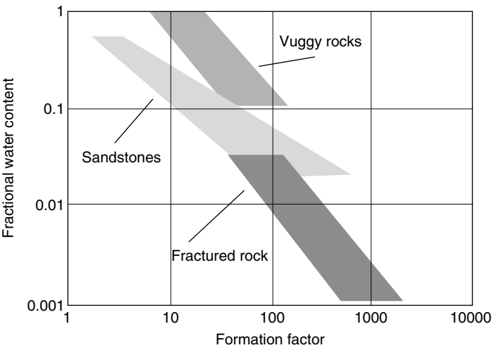
Figure 10.10 Generalized resistivity–water content correlations for three types of pore structure: vugs, intergranular spaces, and fractures.
