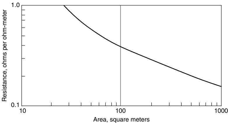
Figure 11.7 The minimum resistance obtainable by connecting a large number of rods in a square of given area in parallel.
