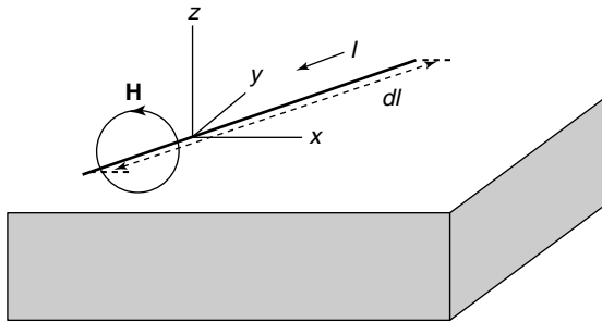
Figure 4.7 Current dipole on the surface of the earth. The length, d\ell , is physically short. The dipole is energized with a current I , providing a dipole moment, I d\ell . The magnetic field, \mathbf{H} , is concentric with the direction of the wire.
