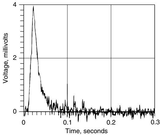
Figure 11.29 Single signal after statistical robusting.
