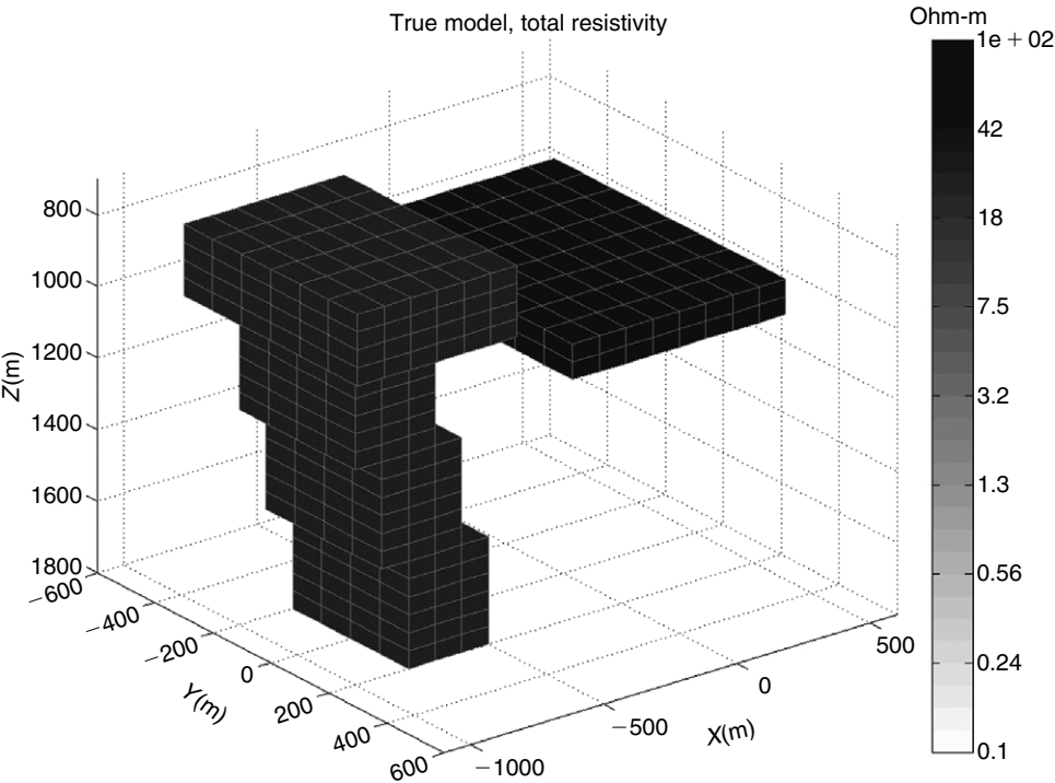
Figure 15.24 A 3D image of true Model 2 of a petroleum reservoir in the presence of a salt dome structure.
