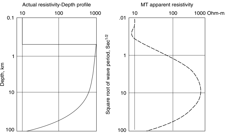
Figure 13.27 Example of the use of the Niblett-Bostick transform to obtain an approximate inversion of an MT sounding curve. The actual resistivity-depth profile is shown on the left. The curve on the right is the Niblett transform of the magnetotelluric curve for the model on the left.
