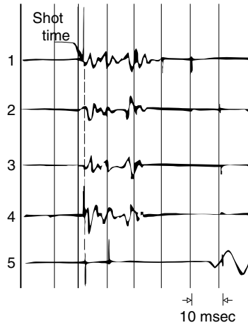
Figure 16.20 Oscillogram of piezoelectric impulses from a quartz vein. Traces 1 through 4 are electrical voltages. Trace 5 is the output of a geophone.
