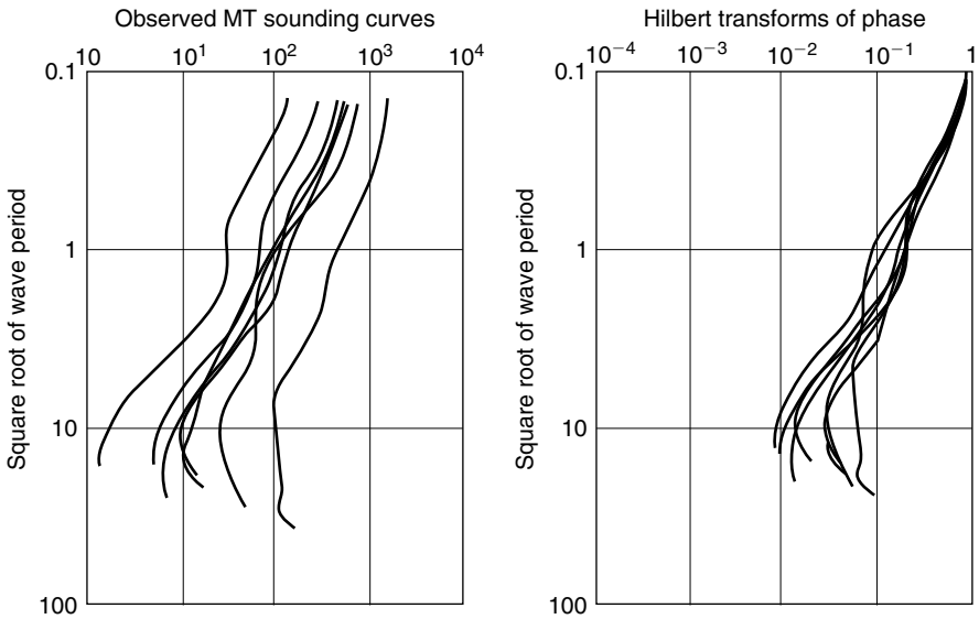
Figure 13.24 Example of the suppression of static shift by using the Hilbert transform of the phase curves to obtain unscaled apparent resistivity curves. On the left, a series of MT sounding curves recorded along a profile in southern British Columbia is shown. The differences between curves is due largely to static shift. Unscaled Hilbert transforms of the corresponding phase curves are shown on the right.
