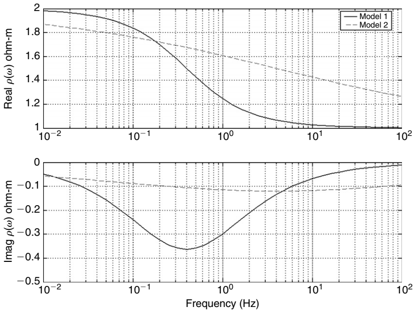
Figure 12.18 Examples of typical complex resistivity curves with the Cole-Cole model parameters. The upper panel shows the real part of the complex resistivity, while the bottom panel presents the imaginary part of the complex resistivity.
