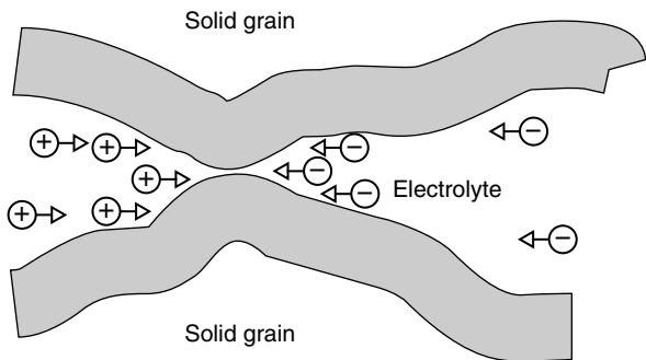
Figure 10.11 Illustration of the action of a bound layer of water in sieving the ions as they move through an electrolyte in the pores of a rock.
