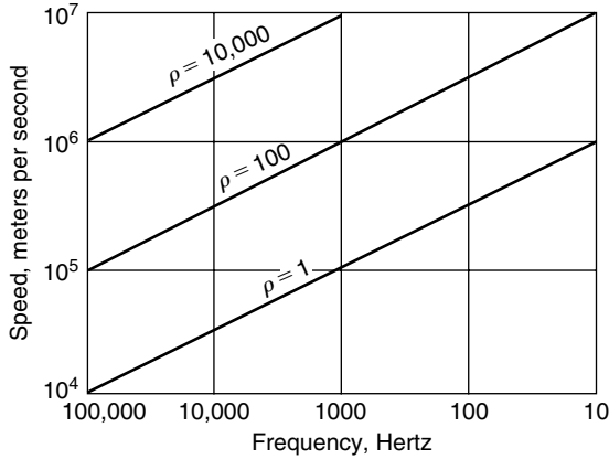
Figure 4.6 Phase velocities of electromagnetic waves traveling through a medium with uniform resistivity.
