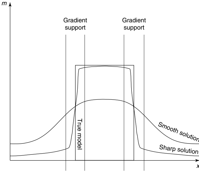
Figure 7.3 Illustration of the principle of the minimum gradient support inversion. A smooth inversion produces a smooth image of a true rectangular model, while the inversion with the minimum gradient support stabilizer generates a sharp image, close to the true model.
