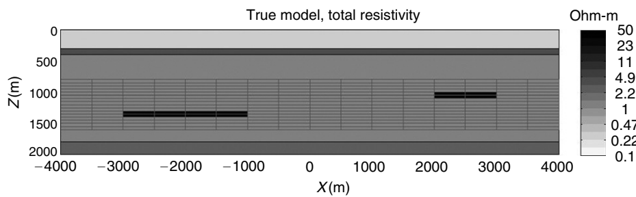
Figure 15.17 Model 1 formed by two resistive reservoirs located at different depths. The area shown with grids defines the extent of the anomalous domain in the inversions.
