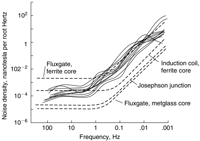
Figure 11.22 Typical noise characteristics of various magnetometers at low frequencies. Noise density curves for the vertical component of the Earth’s magnetic field measured as part of a magnetotelluric survey during the winter months in British Columbia are shown for comparison. Amplitude density is the square root of noise power density.
