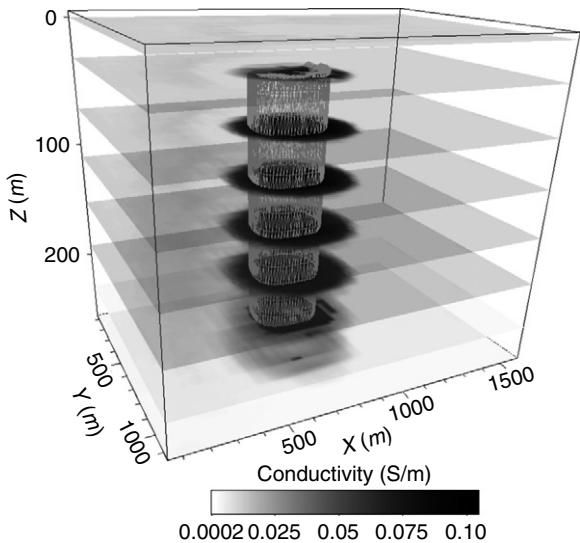
Figure 16.3 The result of rigorous inversion for practical AEM data collected over a kimberlite pipe. The true kimberlite position provided by BHP Billiton is overlain as the cylindrical mesh.
