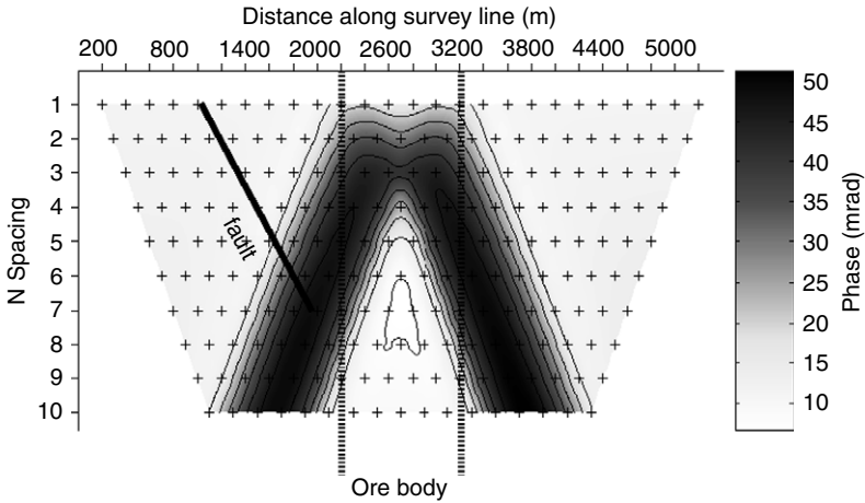
Figure 12.15 Apparent phase pseudosection for 1 Hz data. A phase anomaly due to the ore body is located in the center. One cannot see the influence of the fault in the phase data because it does not produce a strong enough IP response.
