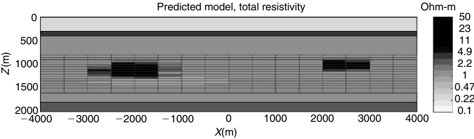
Figure 15.21 Model 1. The vertical section of the result of the inversion of the data contaminated by random noise. The noise level increases linearly from 1% at zero offset up to 7% at 10,000 m offset. The 3D inversion result is obtained with the background model found by 1D inversion. The area shown with grids defines the extent of the anomalous domain in the inversions.
