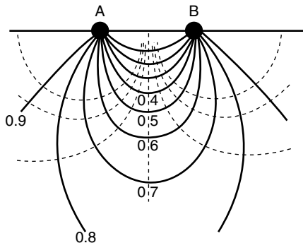
Figure 4.3 Flow of current between two source electrodes implanted in the surface of a uniform half-space. Each of the solid lines separates regions within which one-tenth of the total current flows. The dashed lines are lines of equal voltage.
