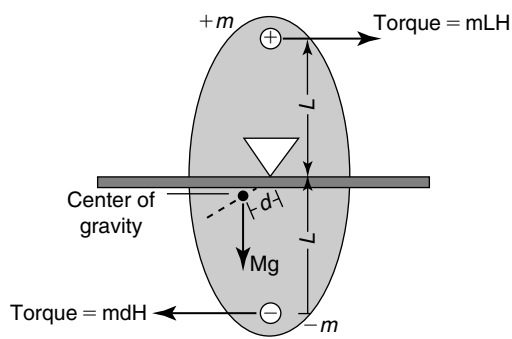
Figure 11.15 Principle of a magnetic balance. A magnetized rod of moment 2mL is balanced at a point slightly offset from its center of gravity. The rod rotates until the gravitational torque about the point of suspension, Mg , balances the torque imposed by the action of the horizontal component of the magnetic field on the magnet, 2mLH . The rotation needed to bring the two torques into balance is a measure of the horizontal component of magnetic field strength, H .
