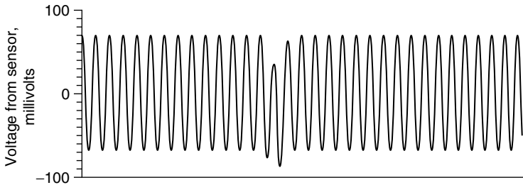
Figure 11.27 Example of wideband (0 to 2000 Hz) recording of the output of a vertical-axis induction loop with an area of 50,000 square meters. The principal noise component is 50 Hz industrial noise. The location is in southern Tuscany, Italy. The presence of the desired signal is indicated by the transient change in the envelope of 50 Hz noise near the center of this record.
