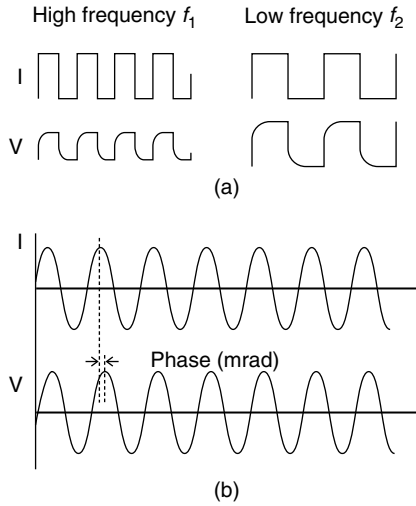
Figure 12.10 Representation of IP effects in the frequency domain. Panel (a) shows percent frequency effect, and (b) the phase difference between the current and the potential.
