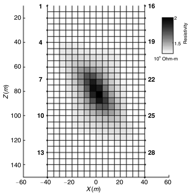
Figure 16.17 A vertical slice through two boreholes of the model obtained as a result of focusing inversion of the crosshole tomographic data.
