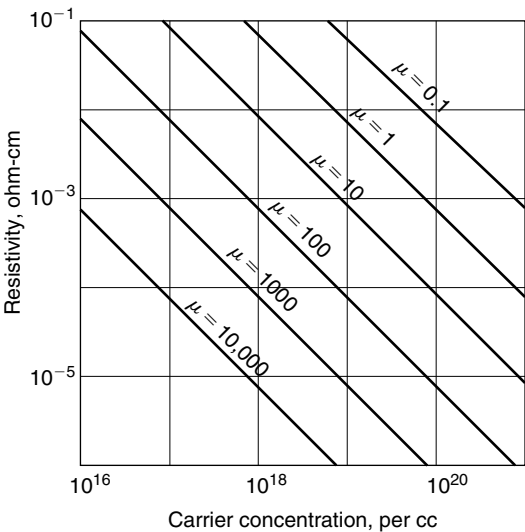
Figure 10.2 Conductivity as a function of free electron concentrations for various values of mobility, \mu , in cgs units.
