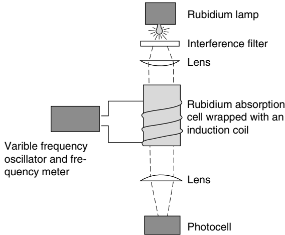
Figure 11.23 Principal elements of an optical pumping magnetometer. Light from a monochromatic rubidium-gas source is used to illuminate a cell containing rubidium gas. Electrons in the rubidium gas are raised to one of two energy states by absorption of energy from the light. These two states correspond to electron orbits that are oriented with or against the ambient magnetic field. These two energy states are slightly different and proportional to the ambient magnetic field. Additional energy is provided to the absorption cell by a coil wrapped around it and energized with an RF current. A servosystem adjusts the frequency so that it provides the energy to cause electrons to move from one to the other of the two excited states. When this occurs, the transmission of the cell is maximum, the photocell detects maximum absorption, and the frequency of the oscillator is a measure of the magnetic field strength.
