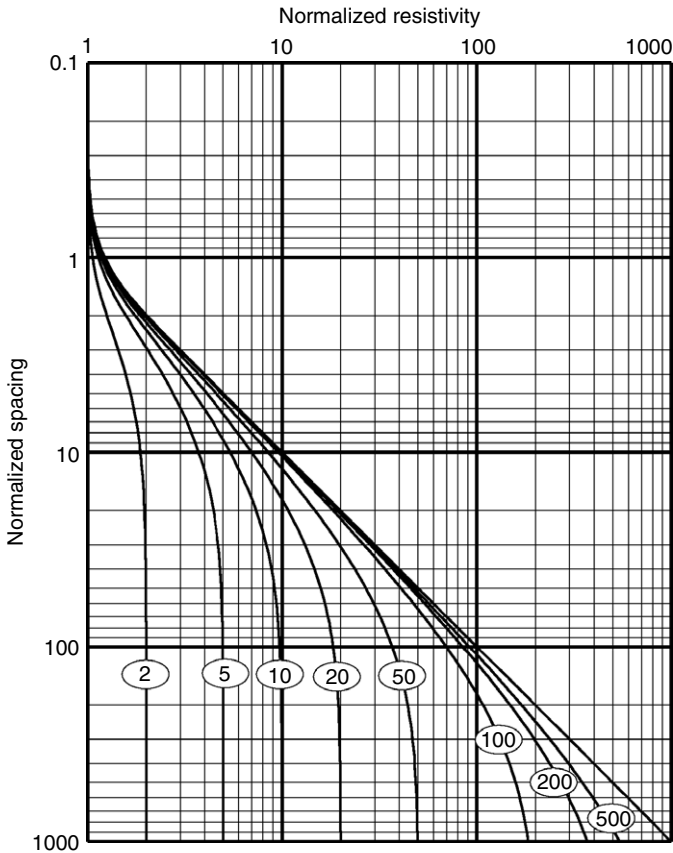
Figure 12.3 Apparent resistivity curves for an expanding Schlumberger array over a sequence of two layers. The upper layer has unit thickness. The contrast in resistivity between the lower and the upper layer is indicated by the label on each curve.
