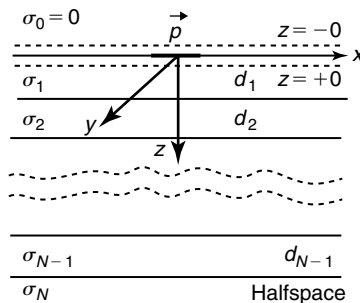
Figure 5.7 Current dipole source on the surface of a layered medium. The dipole is formed by a current passing along a short filament of wire. The moment, \mathbf{p} , is the product of length and current strength.
