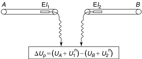
Figure 15.1 A standard design of the marine electrometer.
