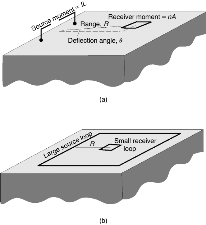
Figure 14.5 Two typical layouts for doing time-domain electromagnetic soundings. a. Grounded wire source method for carrying out time-domain electromagnetic soundings. The grounded source is energized with a square-wave current. The receiver is a sensitive magnetometer, shown here as a vertical-axis induction loop. b. Central loop induction method for carrying out time-domain electromagnetic soundings. The large loop is energized with a square-wave current. The receiver, a sensitive magnetometer, is placed at the center of the source loop.
