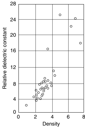
Figure 10.12 Correlation between the relative dielectric constant and density in minerals.
