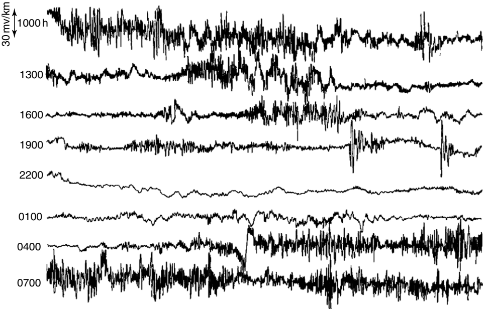
Figure 13.3 Twenty-four hour record of electric field variations (north-south component) in the period band from 1 to 200 seconds recorded at the Cecil Green Observatory at Bergen Park, Colorado. Each raster represents one three-hour interval.
