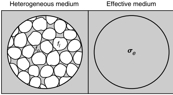
Figure 10.21 The left panel shows a schematic multiphase heterogeneous model of a reservoir rock sample. The right panel represents a corresponding effective-medium model.
