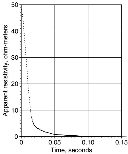
Figure 11.32 Stacked signal after deconvolution.
