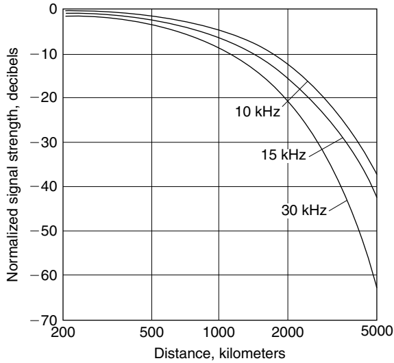
Figure 16.7 Decay of the ground wave for VLF (very low frequency) transmitters operating in the range from 10 to 30 kilohertz (McNeill and Labson, 1991).
