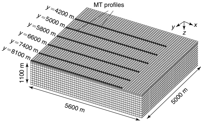
Figure 13.29 Three-dimensional sketch of the inverted area and its discretization for the inversion of the Voisey's Bay area data. The locations of the MT profiles are marked by thick black lines.
