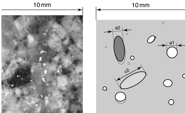
Figure 10.20 Multiphase composite model of general heterogeneous rocks. The left panel, presents a typical slice of a quartz monzonite porphyry (QMP) rock sample. The right panel in the same figure is a schematic multi-phase composite model of the same rock sample with the grains represented by spherical and elliptical inclusions.
