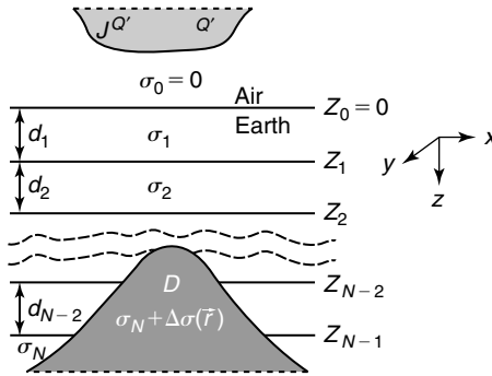
Figure 13.17 Model used in developing the concepts of internal, external, normal, and anomalous parts of an electromagnetic field. In contrast to the model in Figure 13.16, this model includes a region, D , with a resistivity distribution that differs from a one-dimensional resistivity profile.
