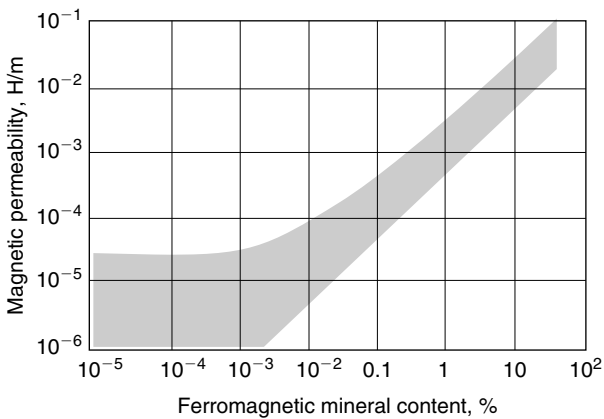
Figure 10.17 Correlation between magnetic permeability and the content of ferromagnetic minerals in intrusive rocks (after Dortman, 1992).
