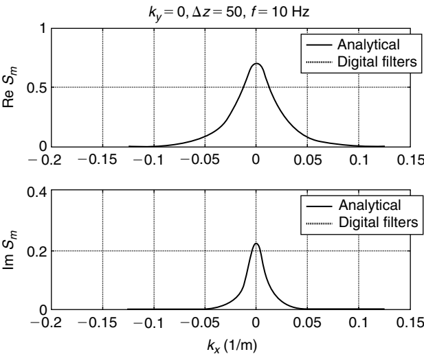
Figure 9.1 Comparison of the spectral characteristic of a digital filter with the analytical spectral characteristic of a migration transformation: f = 10 Hz; \Delta x = \Delta y = 25 m; \Delta z = 50 m; N = L = 50 .
