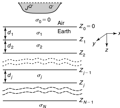
Figure 5.6 Model used in the problem of layered-earth excitation by an arbitrary system of magnetospheric currents.
