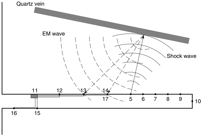
Figure 16.19 Layout of equipment for a piezoelectric survey in an underground working. Shot points are indicated as 5 through 10. Electrodes for detecting the electric field are located at points 12 through 16. A geophone is located at point 17. The recording system is located at point 11.
