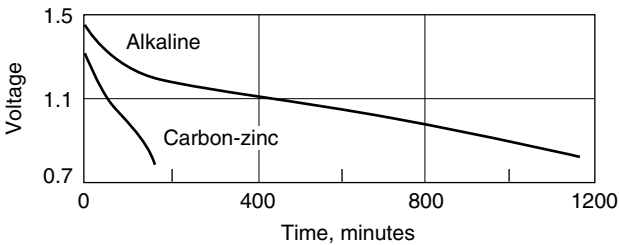
Figure 11.3 Comparison of discharge characteristics for alkaline-manganese and zinc-carbon D-size cells for a half-ampere continuous drain at 21°C.
