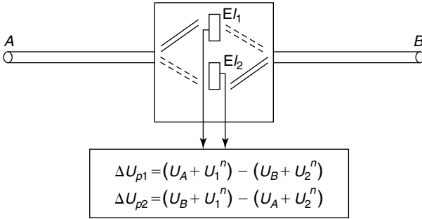
Figure 15.2 Design of a simple water-chopper mechanism used in marine electrometers.
