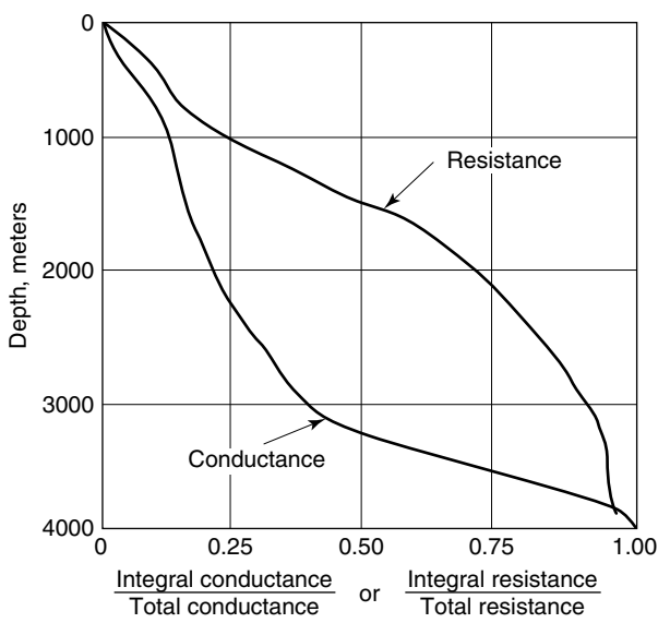
Figure 10.23 Integral resistance and integral conductance curves for a typical layered formation.
