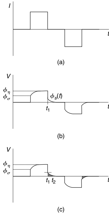
Figure 12.9 Representation of IP effects in the time domain. Panel (a) shows the injected current versus time. The chargeability can be represented as (b), the ratio of potential decay, or (c), the area under the decay curve, to the maximum potential.
