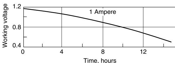
Figure 11.2 Voltage discharge characteristic for an alkaline-manganese primary D-cell battery discharged 24 hours per day.
