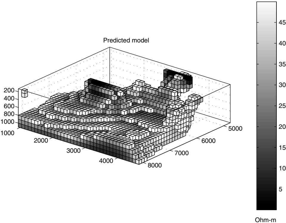
Figure 13.30 Volume image of the inversion results with resistivities below 50 Ohm-m.
