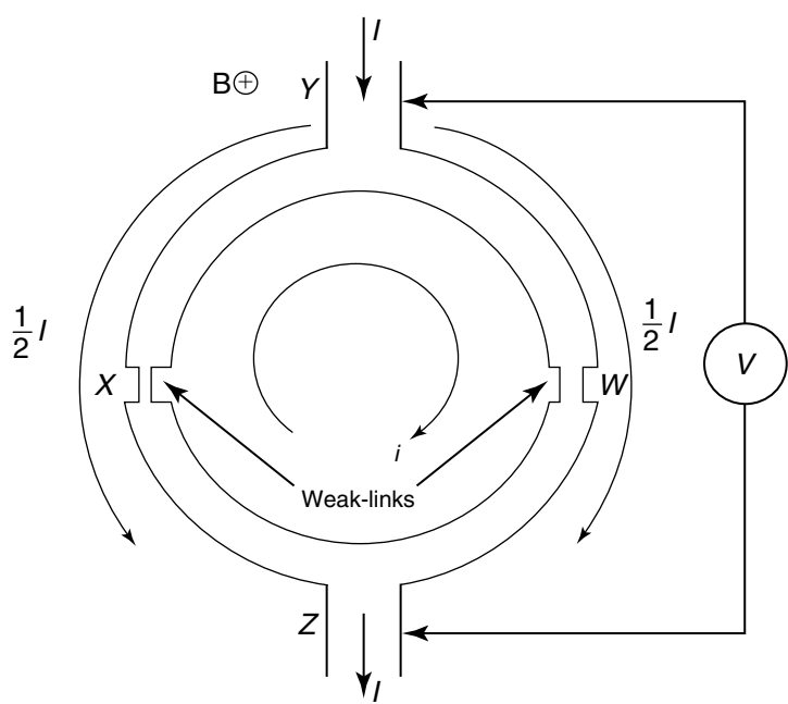
Figure 11.18 Superconducting quantum interference device (SQUID) as a simple magnetometer. The central element of a SQUID is a ring of superconducting material with two weak links, X and W.
