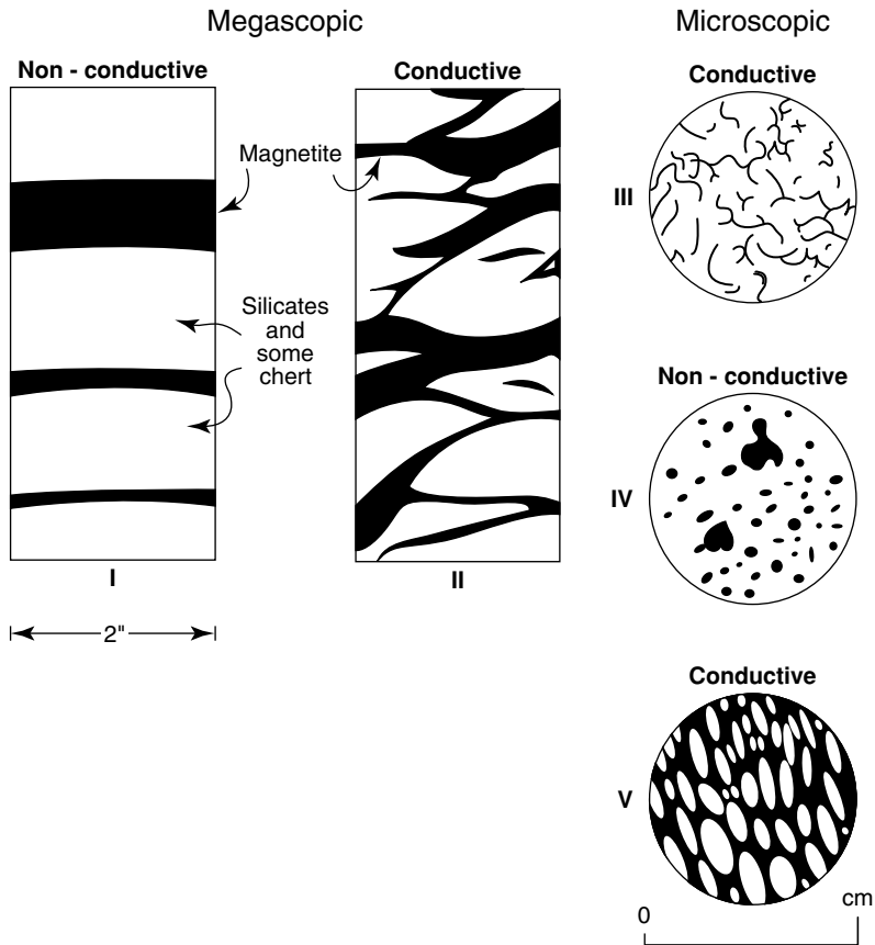
Figure 10.18 Polished sections of a rock showing various crystal habits of hematite.
