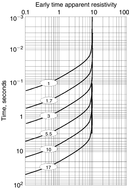
Figure 14.6 Time-domain electromagnetic sounding curves for a uniform earth with a resistivity of 10 ohm-meters. The source-receiver separation (in kilometers) is indicated by the label on each curve.
