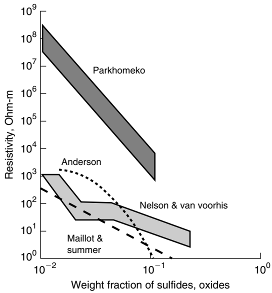
Figure 10.19 Correlations between rock resistivity and the content of conductive minerals as reported by various researchers.
