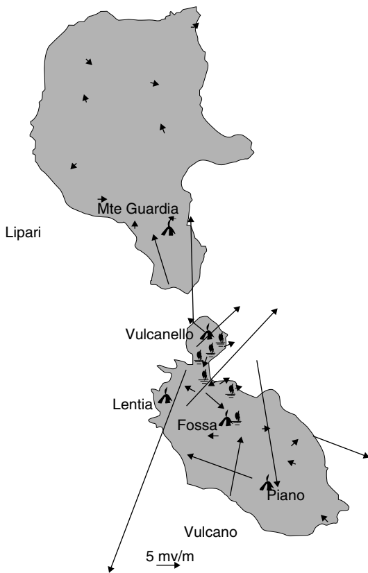
Figure 16.22 Self potential vector survey of Lipari and Vulcano Islands, Italy. Two components of the self potential electric field were observed at selected locations using an orthogonal array of two pairs of electrodes.
