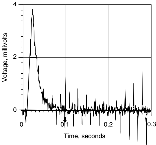
Figure 11.28 Portion of record showing single signal after the 50 Hz noise in Figure 11.26 has been suppressed.
