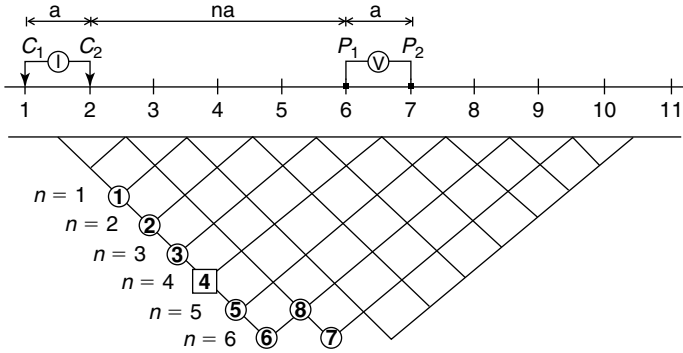
Figure 12.11 Pseudosection representation. The data are plotted at the midpoint of a transmitter and receiver pair versus a separation index, n .
