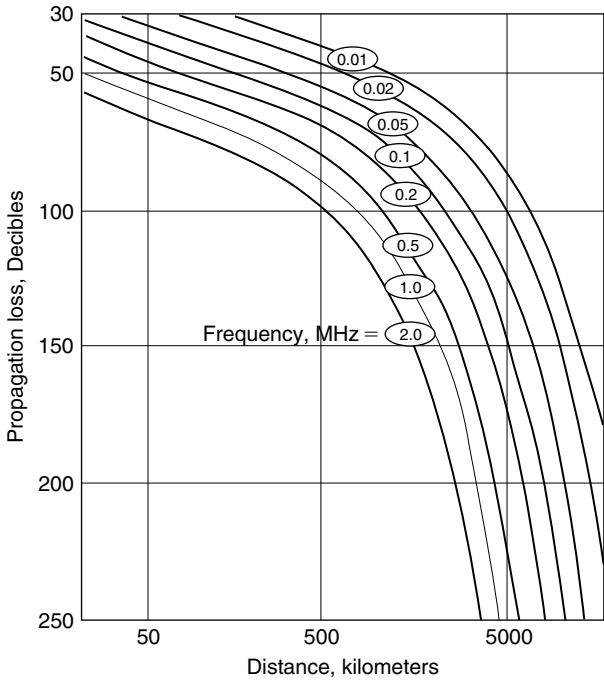
Figure 16.6 Propagation loss for electromagnetic surface waves traveling over a smooth spherical surface. Conductivity is assumed to be 5 S/m and the relative dielectric constant is 80. The source is short vertical antenna. Power radiated is 1 kilowatt, causing an electric field of 300 millivolts per meter at a distance of 1 kilometer.
