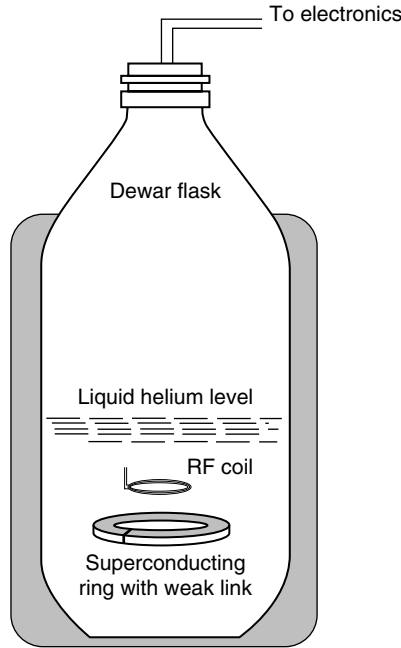
Figure 11.17 Main elements of a Josephson junction magnetometer. The sensing element is a ring of superconducting metal in a bath of liquid helium. The ring has a notch cut in it to form a weak link. Any change in magnetic field will cause a large current to appear in the superconducting ring. The current will increase until it exceeds the saturation current at the weak link. At that point, the resistance at the weak link interrupts the current in the ring. The process continues as long as the magnetic field varies. These changes in current in the ring are detected with a nearby coil, providing a signal which can be used to measure the changing magnetic field.
