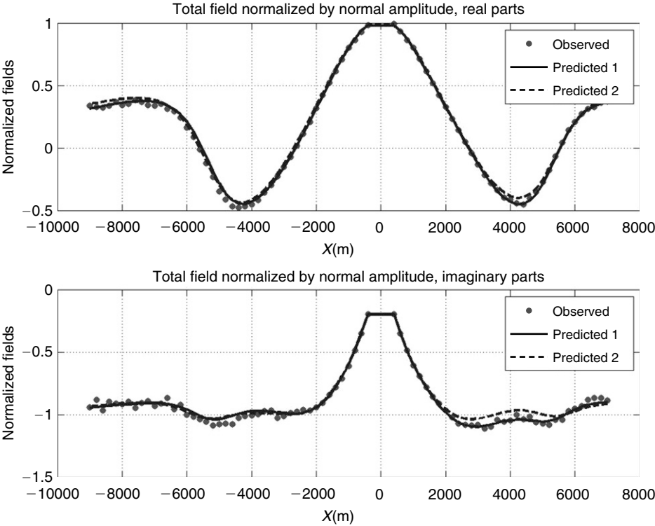
Figure 15.18 Model 1. Plots of the real (top panel) and imaginary (bottom panel) parts of the normalized observed and predicted in-line electric fields E_x at a frequency of 0.25 Hz for receiver #3 ( x = -6,000 m, y = 0 m). The dots show the noisy observed data, while the predicted data for a model obtained by the inversion are plotted by lines. The solid line corresponds to the predicted data (“predicted 1”) obtained by inversion with the true 1-D background model, while the dashed line shows the predicted data (“predicted 2”) computed for 3-D inversion result obtained with the background model found by 1-D inversion.
