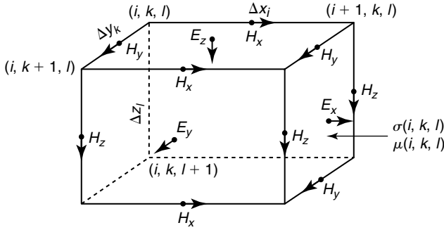
Figure 6.8 The staggered grid for electromagnetic field discretization in the electromagnetic potential method. The normal components of electric field \mathbf{E} are defined at the centers of the cell faces, while the tangential components of magnetic field \mathbf{H} are defined on the cell edges.
