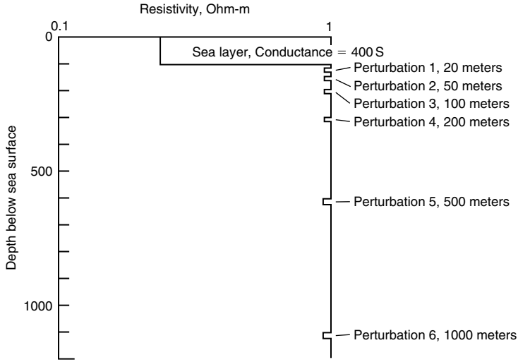
Figure 15.8 Model illustrating a resolution analysis for a shallow-water electrical survey.
