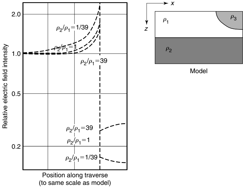
Figure 13.21 Behavior of a static electric field for a two-layer model with a hemispheroidal conductive pod in the surface layer. The pod has a resistivity 1/9 of that of the rest of the surface layer.
