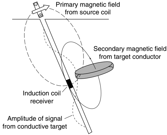
Figure 16.14 One concept of borehole assisted electromagnetic surveying. A transmitter is placed at the surface of the earth near a borehole, providing a field which induces currents in underground conductors. A receiving coil is moved along the borehole, detecting the presence of a conductor by recording the secondary magnetic field from the induction currents in it.
