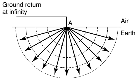
Figure 4.2 Geometric behavior of current flow from a point source on the surface of a uniform earth. The current flows with radial symmetry as shown by the solid arrows. Surfaces of equal voltage are hemispheres as shown by the dotted lines.
