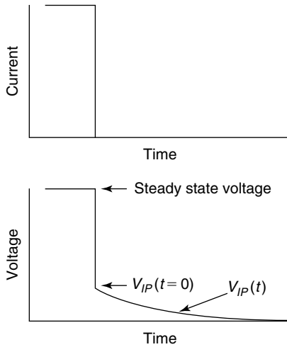
Figure 10.1 Characterization of geophysical induced polarization.
