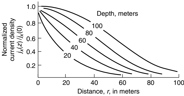
Figure 4.4 Plots of the normalized current density, j_x(z)/j_x(0) , versus depth for various separations, L .
