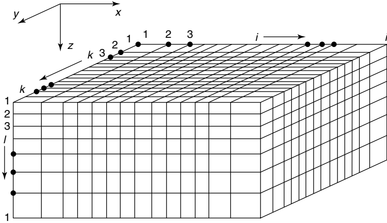
Figure 6.4 The model region is discretized into a number of prisms. The indices i , k , and l are used to number the grid point in the x , y , and z directions, respectively. Electromagnetic parameters, \sigma , \mu , and \varepsilon , are assumed to be constant within each elementary prism.
