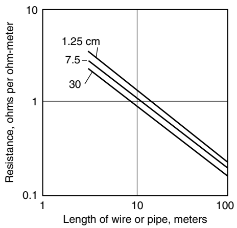
Figure 11.9 Grounding resistance of a length of wire or metal pipe buried at a depth of 1 meter. The label on each curve is the diameter of the conductor.
