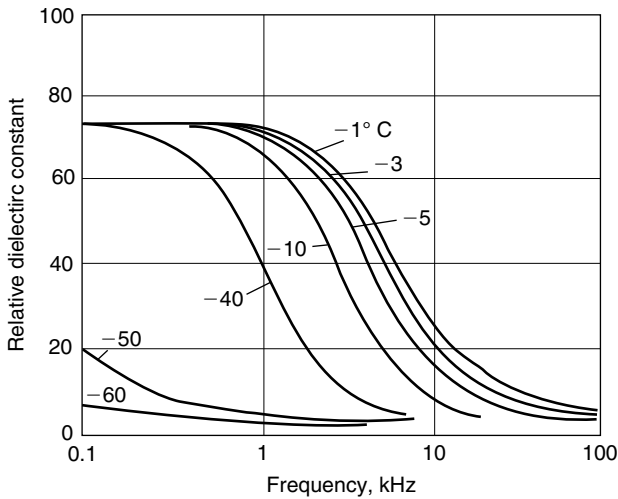
Figure 10.14 Relative dielectric constant of ice at various temperatures.
