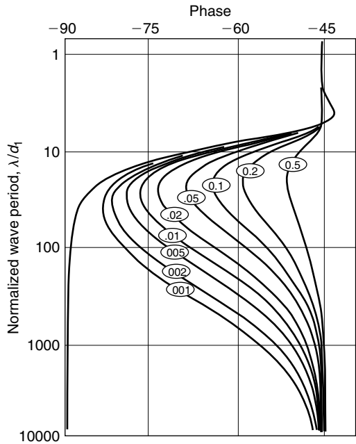
Figure 13.8 Phase of the magnetotelluric apparent resistivity curves. The contrast in conductivity between the second layer and the first is specified by the label on each curve.
