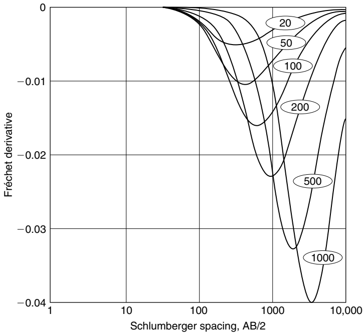
Figure 15.9 A set of curves for the maximum change in apparent resistivity caused by the presence of the perturbing thin layer at various depths beneath the seafloor for the Schlumberger array deployed at the surface of a sea with various depths (conductances).
