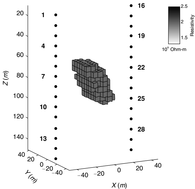
Figure 16.18 A 3-D view of the inversion result with volume rendering. The cut-off level for this image is equal to 100 Ohm-m. This means that only the cells with a value of anomalous resistivity greater than 100 Ohm-m are displayed.
