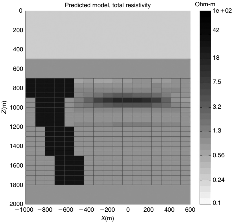
Figure 15.25 Model 2. The vertical section of the result of the inversion of the data contaminated by random noise. The noise level increases linearly from 5% at zero offset up to 10% at 3,000 m offset. The true salt dome background conductivity model is used in the inversion. The area shown with grids defines the extent of the anomalous domain in the inversions.
