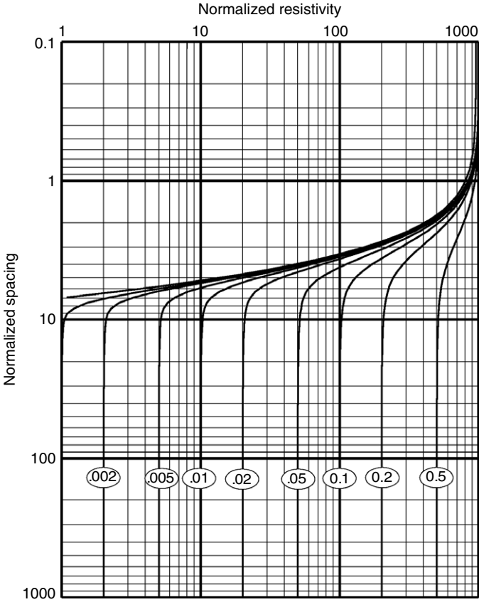
Figure 12.4 Apparent resistivity curves for an expanding Schlumberger array over a two-layer sequence. The upper layer has unit resistivity and unit thickness. The contrast in resistivity between the lower layer and the upper layer is indicated by the number on each curve.
