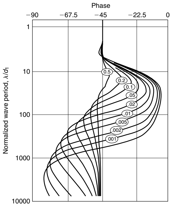
Figure 13.13 Phase for the magnetotelluric apparent resistivity curves shown in previous Figure.
