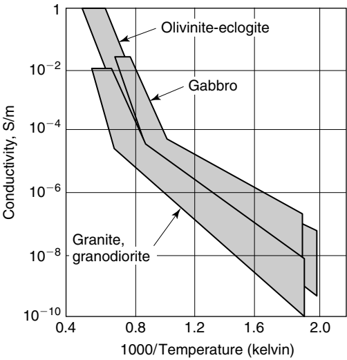
Figure 10.5 Generalized Arrhenius plots of conductivity as a function of inverse temperature for igneous rocks with diverse chemical makeup.
