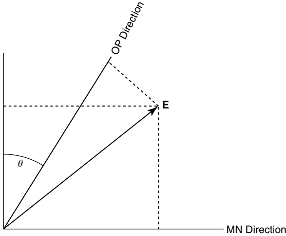
Figure 11.12 Often, in field operations, the electric field is measured in terms of two components which are not orthogonal. The magnitude and direction of the vector can be determined with this sketch of the various projections of the vector on the real field directions and on a set of orthogonal axes.
