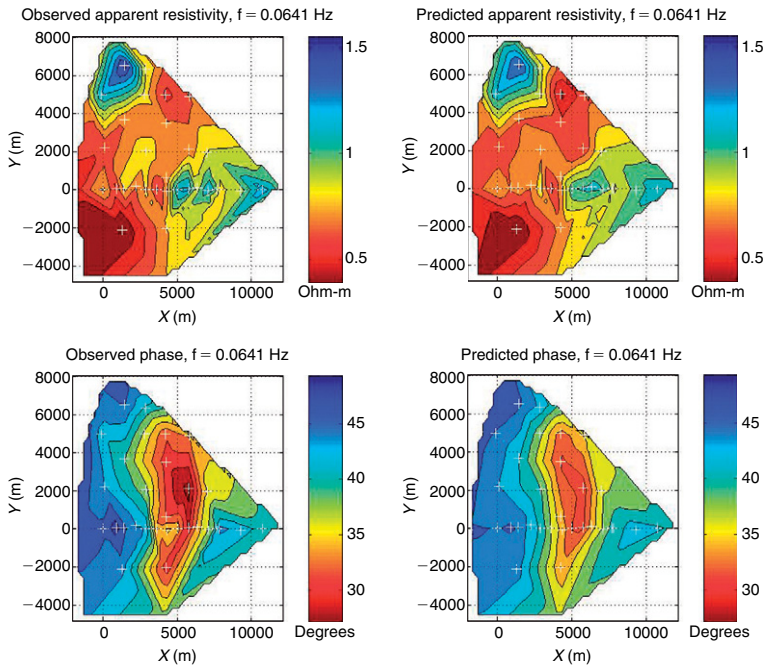
Figure 15.6 Plots of the observed (the left-hand panels) and predicted (the right-hand panels) apparent resistivity and phase for the MT data collected in the MT sites at the Gemini Prospect area.
