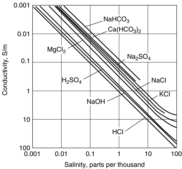
Figure 10.6 Dependence of the conductivity of an electrolytic solution on the amount of salt in solution at a temperature of 18°C.
