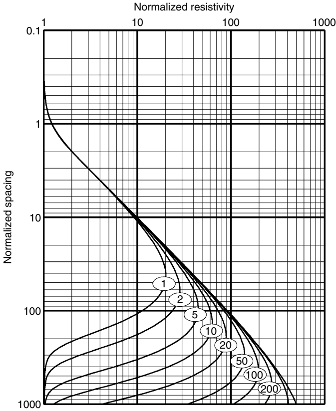
Figure 12.6 Apparent resistivity curves for an expanding Schlumberger array over a sequence of three layers. The upper and lower layers have unit resistivity, while the middle layer has a resistivity of 1000 units. The thickness of the middle layer, in units, is indicated by the label on each curve.
