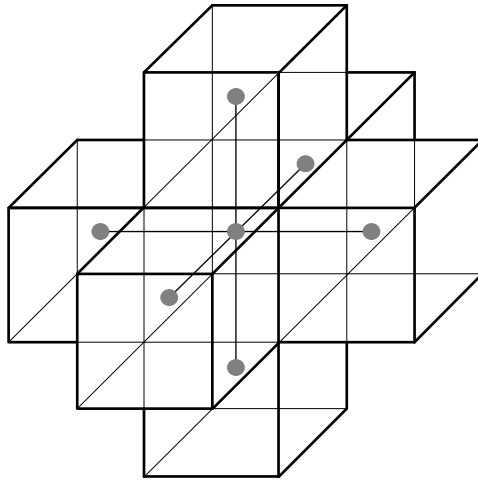
Figure 6.7 Within the framework of the balance method, the resulting stencil for electric field \mathbf{E} has seven points, located at the center of the prismatic conductivity cell, and at the centers of six adjacent cells.
