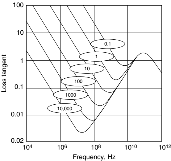
Figure 16.11 Dielectric loss in water. Loss tangent as a function of frequency for saline water with various resistivities as indicated by the labels on the curves. The local maximum in loss tangent at high frequencies is caused by rotational polarization of water molecules.
