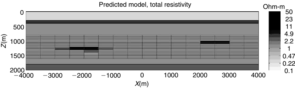
Figure 15.20 Model 1. The vertical section of the result of the inversion of the data contaminated by random noise. The noise level increases linearly from 1% at zero offset up to 7% at 10,000 m offset. The true layered-earth background conductivity model is used in the inversion. The area shown with grids defines the extent of the anomalous domain in the inversions.
