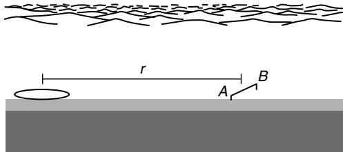
Figure 15.11 Simple sea-bottom survey design: measurement of the electric field originating from a horizontal loop source on the seafloor.
