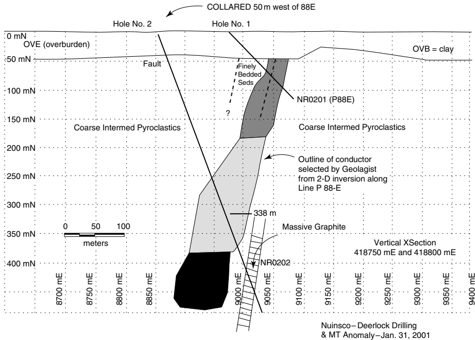
Figure 13.34 A geological cross-section based on the results of two drill holes in in Deerlock Property (courtesy of Phoenix Geophysics).
