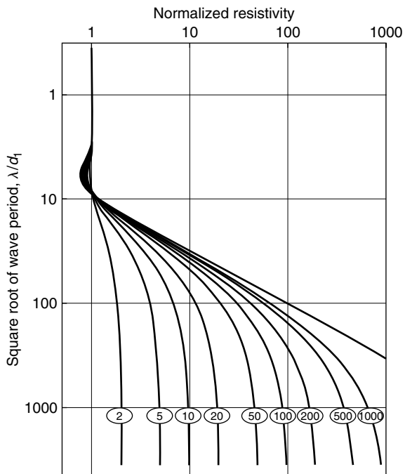
Figure 13.7 Magnetotelluric sounding curves for a two-layer sequence in which the second layer is more resistive than the first. The contrast in resistivity between the second layer and the first is specified by the label on each curve. The normalized wave period is \lambda_1/d_1 . The normalized resistivity is \rho_2/\rho_1 .
