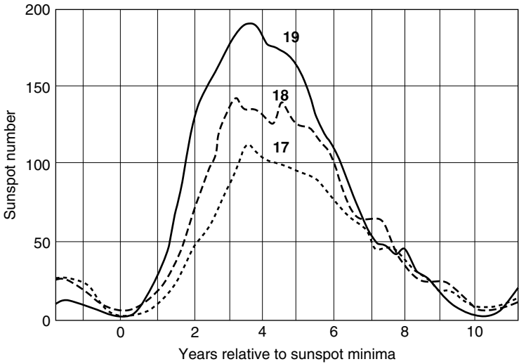
Figure 13.5 Sunspot numbers that occurred during sunspot cycle 17 (1933–1944), cycle 18 (1944–1954), and cycle 19 (1954–1964).
