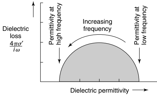
Figure 10.15 A Cole-Cole plot of the frequency-dependent behavior of the dielectric permittivity in a complex plane.
