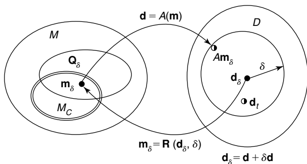
Figure 7.4 The stabilizing functional selects from a set of the possible solutions, Q_\delta , a solution, \mathbf{m}_\delta , which at the same time belongs to the correctness set M_C .
