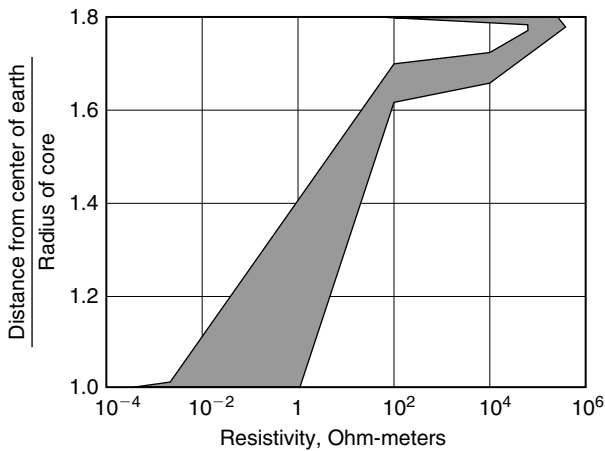
Figure 10.24 Summary of estimates of the resistivity-depth profile in the earth from the bottom of the mantle to the surface.
