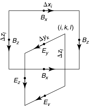
Figure 6.6 The concept of electric and magnetic loops in a staggered grid in discretizing Maxwell’s equations (according to Wang and Hohman, 1993). The electric loop is formed by four \mathbf{E} components parallel to the edges of one face of a prism, and the magnetic loop is composed of four adjacent \mathbf{B} components.
