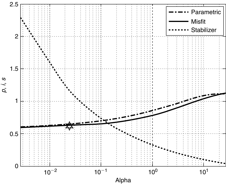
Figure 7.5 Illustration of the principle of optimal regularization parameter selection. The plots show the behavior of the misfit functional, parametric functional, and a stabilizer versus the logarithm of the regularization parameter, \alpha .
