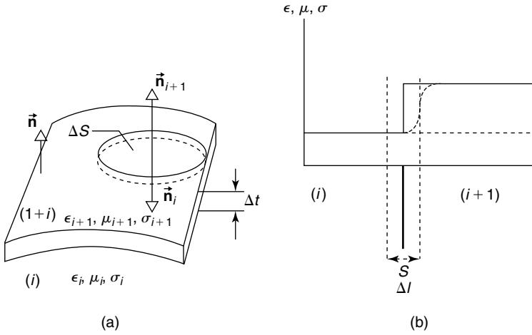
Figure 3.3 Formulation of the boundary conditions for electromagnetic field: the surface S separating medium (i) from medium (i+1) is replaced with a very thin transitional layer with a thickness \Delta\ell in which the parameters \epsilon , \mu , and \sigma vary rapidly but continuously.
