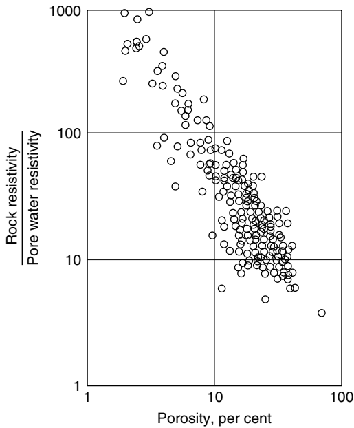
Figure 10.9 Scatter plot of pairs of resistivity and porosity values for water-saturated sandstones.
