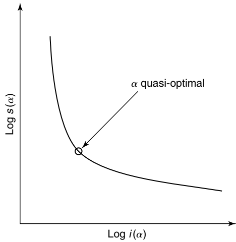
Figure 7.6 The L curve represents a simple curve for all possible \alpha of the misfit functional, i(\alpha) , versus the stabilizing functional, s(\alpha) , plotted in log-log scale. The distinct corner, separating the vertical and the horizontal branches of this curve, corresponds to the quasi-optimal value of the regularization parameter \alpha .
