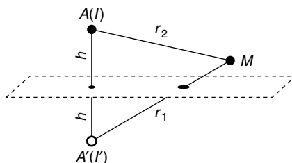
Figure 5.5 Geometric definition of a Kelvin image.
