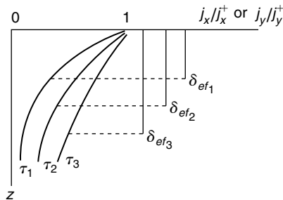
Figure 5.11 Change in current density as a function of depth for several instants in time.
