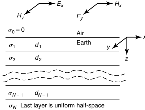
Figure 5.1 A model of a plane electromagnetic wave in a horizontally stratified medium. The electromagnetic field is excited in the earth by a downward-travelling plane electromagnetic wave.
