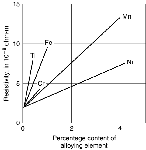
Figure 10.3 Resistivity of copper-based binary alloys with small amounts of metals other than copper in solution.
