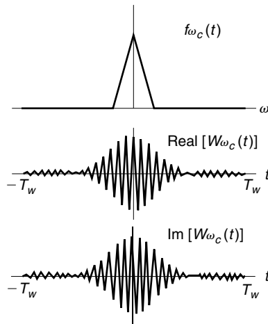
Figure 13.19 Frequency and time domain characterization of a filter response used in processing of magnetotelluric data.
