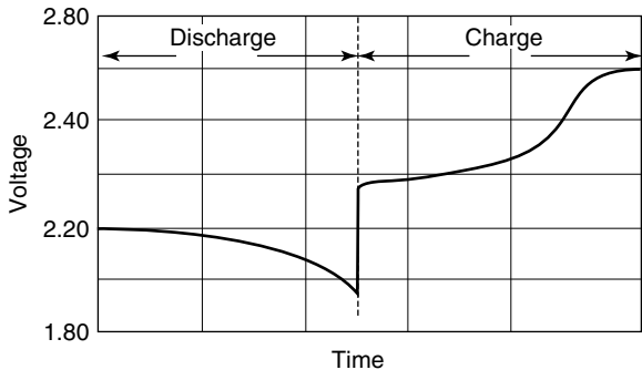
Figure 11.4 Charge and discharge cycles for a lead/acid storage battery.
