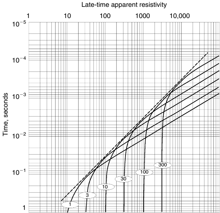
Figure 14.9 Apparent resistivity curves computed using the late-time asymptotic expression for a uniform earth. The separation from transmitter to receiver is 1000 meters. The resistivity of the earth is shown on the label on each curve.
