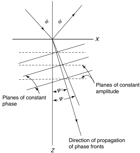
Figure 16.10 Reflection and refraction at the surface of a lossy medium.
