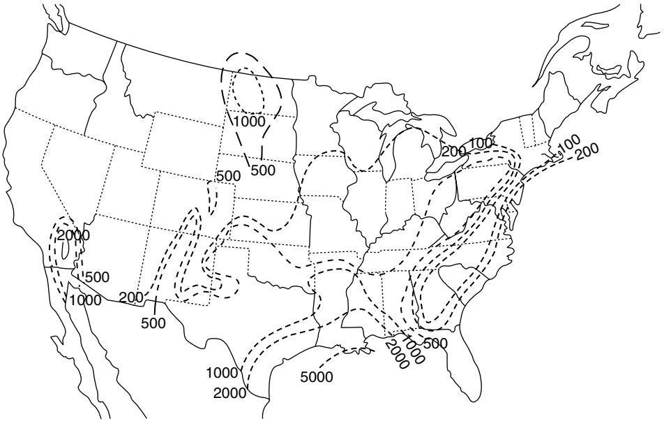
Figure 10.25 Total conductance in major sedimentary basins of the United States.
