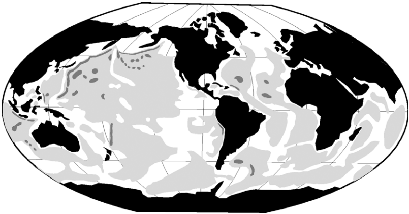
Figure 10.27 Conductivity of the World’s Ocean. Areas in black are the continents. Areas in white are oceanic areas with a conductance of less than 12 kilosiemens. Lightly shaded areas have a conductance between 12 and 18 kilosiemens. The small areas with darker shading have a conductance greater than 18 kilosiemens.
