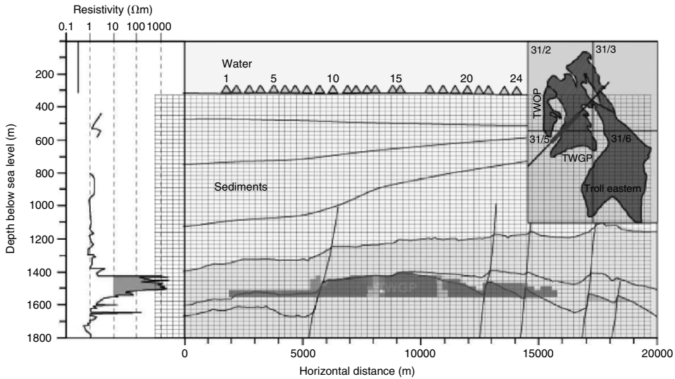
Figure 15.29 Cross section of the result of iterative migration overlapping on the geological cross section along the MCSEM survey line in the Troll West Gas Province (TWGP), offshore Norway.
