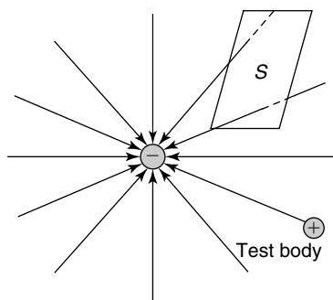
Figure 1.1 Force lines of the electric field of a negatively charged sphere.
