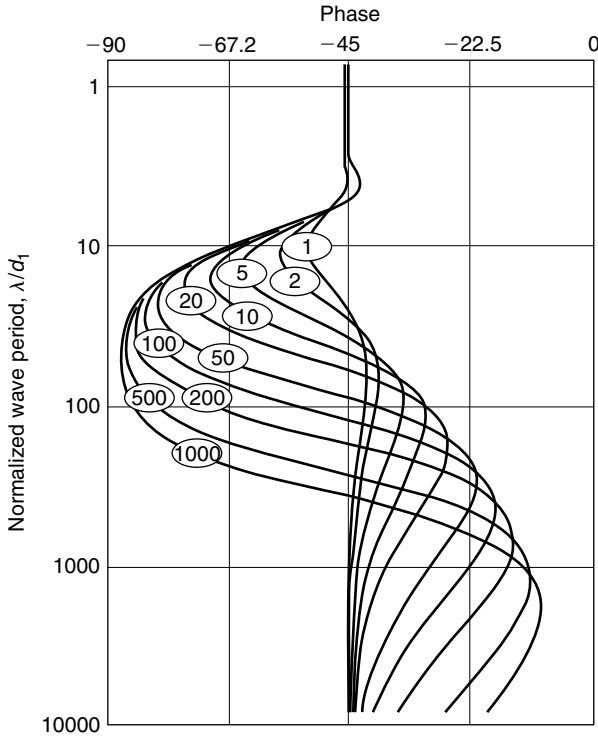
Figure 13.15 Phase of the magnetotelluric apparent resistivity curves of the previous Figure.
