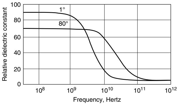
Figure 10.13 Molecular polarization in liquid water at a temperature of 1°C.
