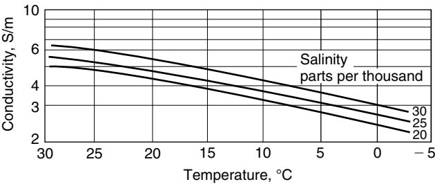
Figure 10.26 Conductivity of sea water as a function of total salinity and temperature.
