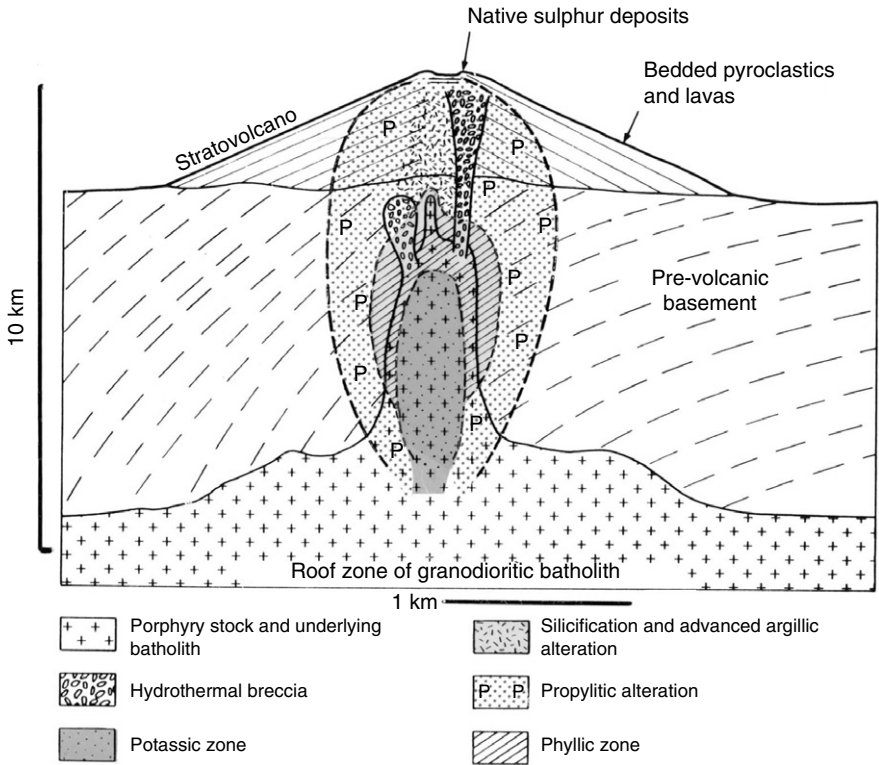
Figure 12.12 Porphyry genesis: a geologic overview of the creation of a porphyry deposit (after Sillitoe, 1973).
