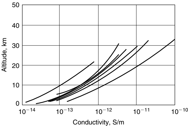
Figure 10.28 Conductivity profiles through the lower part of the atmosphere.
