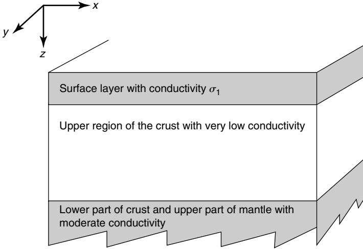
Figure 5.2 A horizontally layered model of the Earth's crust and upper mantle consisting of three zones with characteristic conductivity values.
