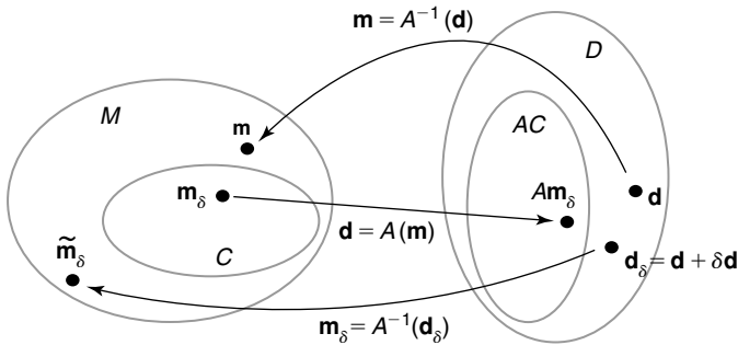
Figure 7.1 A quasi-solution, \mathbf{m}_\delta , is selected from the correctness set C under the condition that its image, A(\mathbf{m}_\delta) , is the closest element to the observed noisy data, \mathbf{d}_\delta , from the subset AC : \|A\mathbf{m}_\delta - \mathbf{d}_\delta\|_D = \inf_{\mathbf{m} \in C} \|A\mathbf{m} - \mathbf{d}_\delta\|_D .
