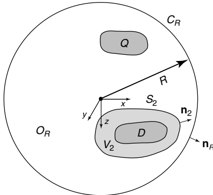
Figure 6.1 Derivation of Poynting's theorem and energy inequality for an anomalous field.
