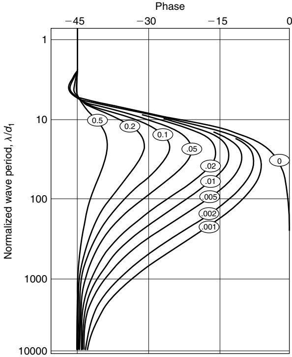
Figure 13.10 Phase of the magnetotelluric apparent resistivity curves. The contrast in resistivity between the second layer and the first is specified by the label on each curve.
