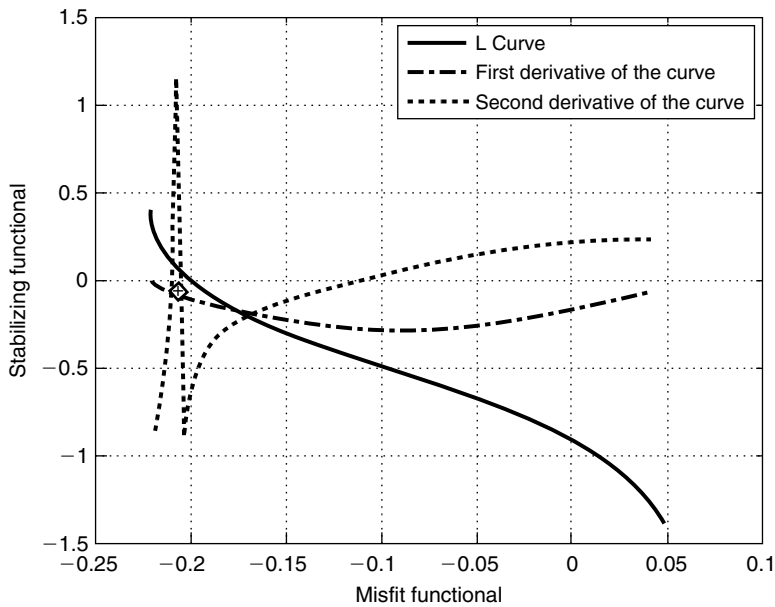
Figure 7.7 L-curve plot for selection of the quasi-optimal regularization parameter \alpha . The star dot shows the point where the curvature of the curve is greatest, corresponding to the quasi-optimal value of the regularization parameter \alpha .
