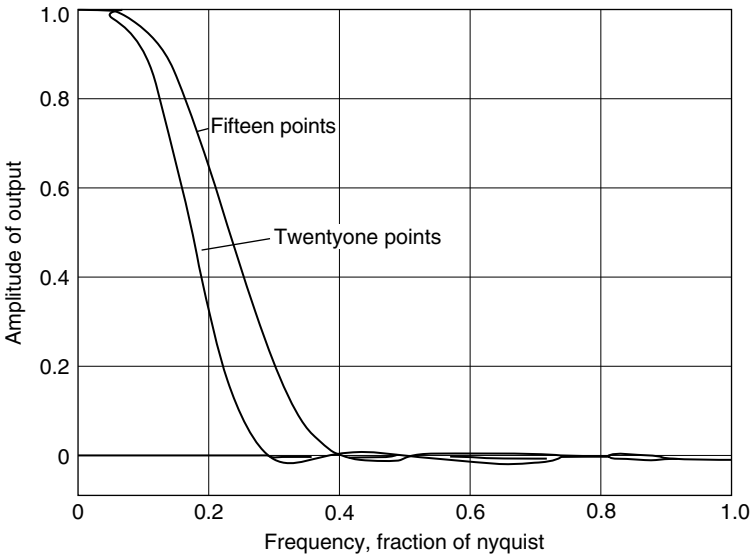
Figure 11.26 Frequency responses of Spencer’s 15- and 21-point smoothing operators.
