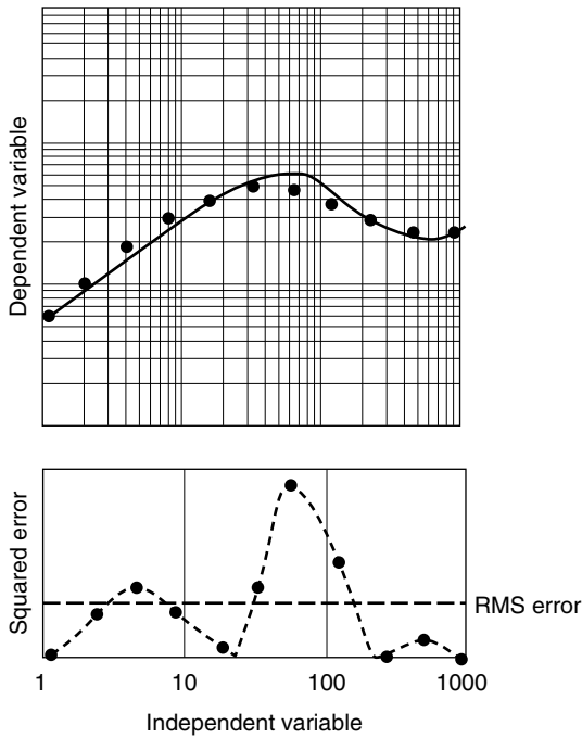
Figure 7.2 Definition of RMS error measure for a curve plotted in logarithmic coordinates. Errors of individual points are measured as the distance between a data point and a fitted curve when both are plotted to logarithmic coordinates.
