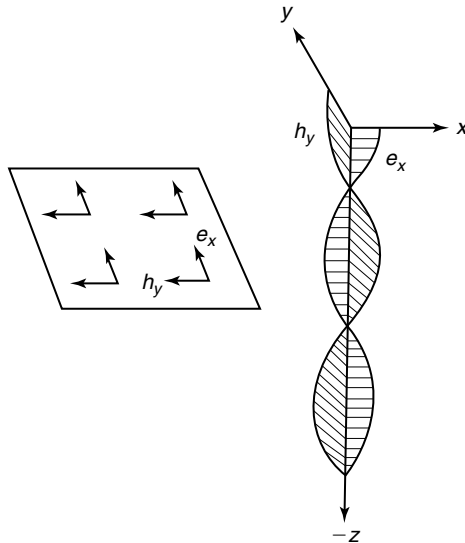
Figure 4.5 In a downward-traveling plane electromagnetic wave, the magnetic and electric vectors lie in horizontal planes.
