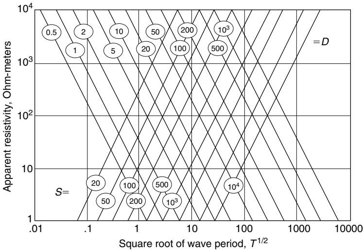
Figure 13.26 Dimensioned asymptotes to magnetotelluric sounding curves for two-layer cases with a perfect insulator at depth ( S -curves) or a perfect insulator at depth ( D -curves).
