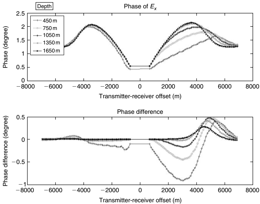
Figure 15.15 Plots of the electric field phase versus offset for a model with the resistive reservoir located at different depths.
