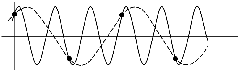
Figure 11.24 Nature of aliasing in sampling. If a monochromatic function is sampled at a rate of two samples per cycle or less, that function cannot be distinguished from another monochromatic function with a longer period which will also pass through the sampled points.
