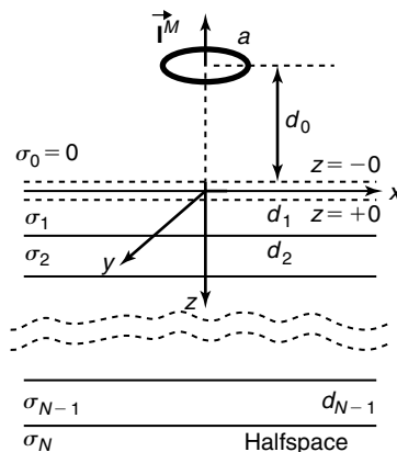
Figure 5.8 Vertical-axis magnetic dipole raised to a height d_0 above a stratified earth. The magnetic dipole is formed by a current-carrying loop of wire with an effective area, a , and a magnetic moment \mathbf{I}^M .
