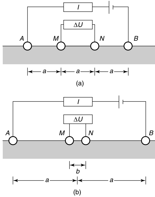
Figure 12.2 The Wenner (a) and Schlumberger (b) electrode arrays.
