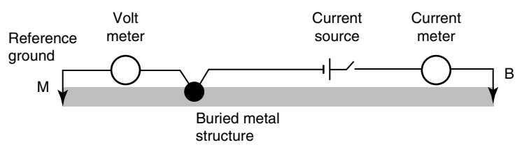
Figure 11.10 Three-terminal circuit to determine the approximate single-terminal resistance of a ground. Here, we wish to determine the grounding resistance of a preexisting system. A low frequency or direct current is driven through the ground to a return, B, while the voltage between the metal structure and a reference ground, M, is measured. The resistance is the ration of this voltage to the current.
