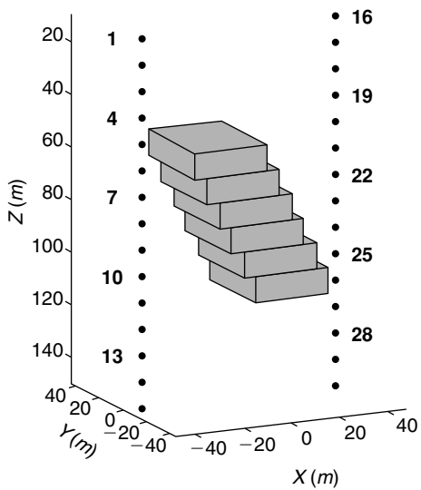
Figure 16.15 Model of a dipping resistive body with a resistivity of 500 Ohm-m in a 20 Ohm-m conductive background.
