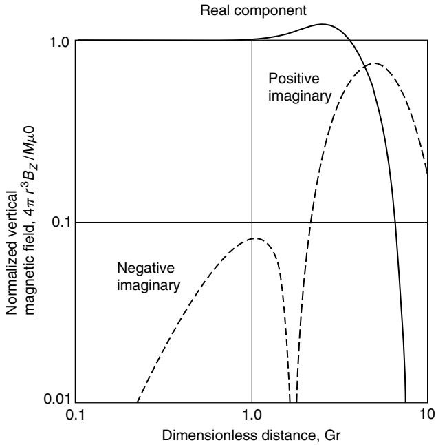
Figure 14.2 Normalized mutual impedance for two vertical-axis loops lying on the surface of a uniform half-space as a function of the normalized separation between the loops. The plots show the absolute values of the real and imaginary parts of the normalized mutual impedance in logarithmic scale.
