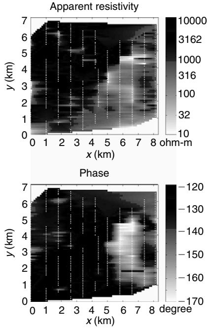
Figure 13.28 Maps of the observed Z_{yz} apparent resistivities and phases at f = 96 Hz over the Voisey's Bay area. The white dots mark the observation sites.
