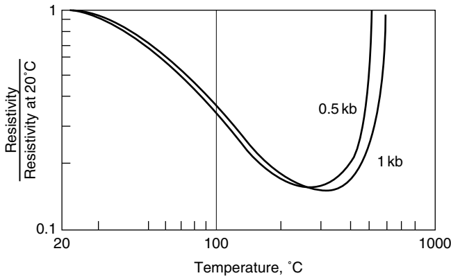
Figure 10.8 Relative change in the resistivity of the electrolyte with temperature, normalized to the resistivity at 20°C.
