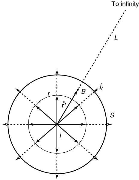
Figure 4.1 A scheme of the current distribution of a point source in an isotropic and homogeneous medium with constant conductivity, \sigma .
