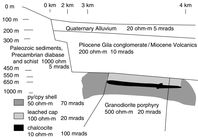
Figure 12.13 Southwest US copper porphyry geoelectrical model (J. Inman, pers. commun.). The figure presents basic scale information, geologic units, and geoelectrical properties. Note that there is a normal fault on the left side of the model.
