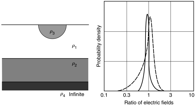
Figure 11.14 Probability distribution of electric field strengths measured in the vicinity of a hemispherical surface inclusion of higher or lower resistivity. The solid curve is the distribution for a resistive inclusion (9:1) and the dashed line is the distribution for a conductive inclusion (1:1/9). The electric field ratio is the normalization of the electric field with the inclusion present to that when it is absent. Note the wider distribution function and the skewing toward lower electric fields in the case of a conductive inclusion.
