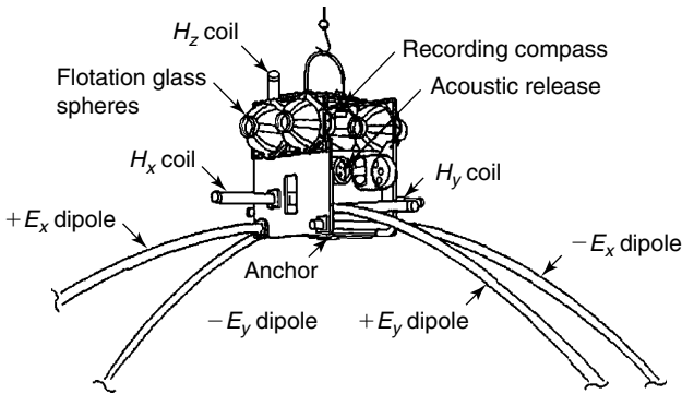
Figure 15.3 Typical design of a sea-bottom MT instrument. (Modified from Costable et al., 1998).
