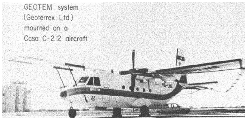
Figure 16.1 Aircraft carrying airborne electromagnetic system.
