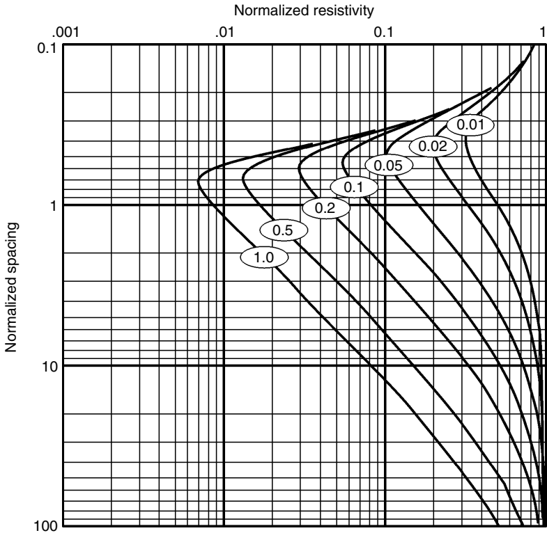
Figure 12.5 Apparent resistivity curves for an expanding Schlumberger array over a sequence of three layers. The upper and lower layers have unit resistivity, while the middle layer has a resistivity of 0.001 unit. The thickness of the middle layer, in units, is indicated by the label on each curve.
