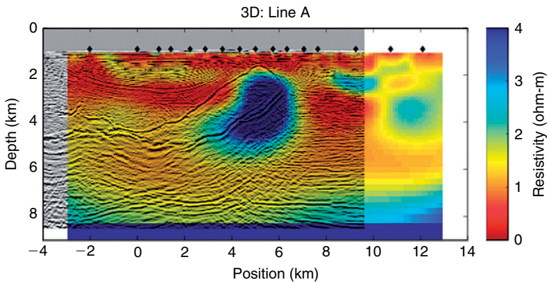
Figure 15.7 A vertical cross section of 3-D focusing inversion results provided over line A. The observational profile is oriented from southwest (left) to northeast (right). The MT site locations are shown as black diamonds. The resistivity distribution in the inverse model is shown on a linear scale. The inverse geoelectrical model is overlapped with the depth-migrated seismic reflections from a 3-D seismic survey.
