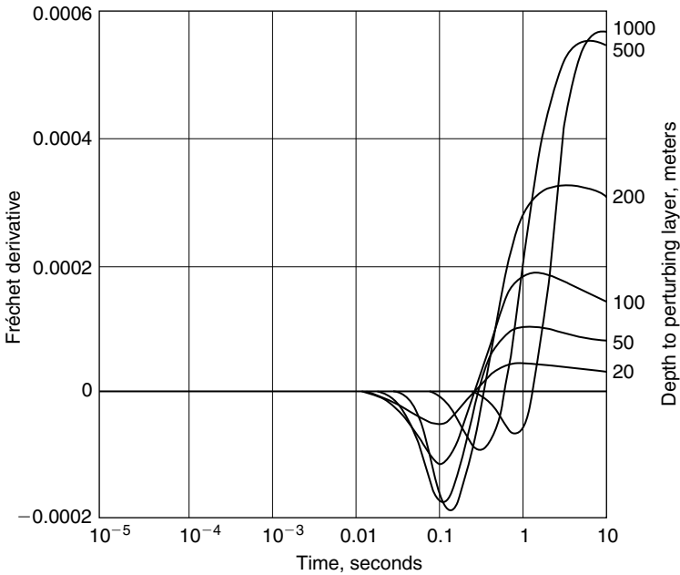
Figure 15.10 Fréchet derivative curves for a continental shelf sedimentary model. The ocean was assigned a depth of 100 meters and a resistivity of 0.25 ohm- meters. The sea floor was assigned a uniform resistivity of 1 ohm-meter. A perturbing layer with a resistivity of 0.9 ohm meters and a thickness of 10% of the depth was inserted at various depths beneath the sea floor as indicated on each curve. The system modeled is a wire-loop TDEM sounding system with a source receiver separation of 1000 meters.
