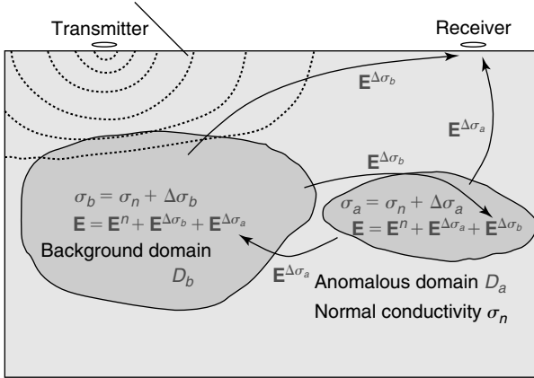
Figure 6.3 A sketch of 3D geoelectrical model with horizontally layered (normal) conductivity, \sigma_n , inhomogeneous background conductivity, \sigma_b = \sigma_n + \Delta\sigma_b , within a domain D_b , and anomalous conductivity, \Delta\sigma_a , within a domain D_a . The EM field in this model is a sum of the normal fields, \mathbf{E}^n , \mathbf{H}^n , generated by the given source(s) in the model with normal distribution of conductivity, \sigma_n , a variable background effect, \mathbf{E}^{\Delta\sigma_b} , \mathbf{H}^{\Delta\sigma_b} , produced by the inhomogeneous background conductivity, \Delta\sigma_b , and the anomalous fields, \mathbf{E}^{\Delta\sigma_a} , \mathbf{H}^{\Delta\sigma_a} , due to the anomalous conductivity distribution, \Delta\sigma_a .
