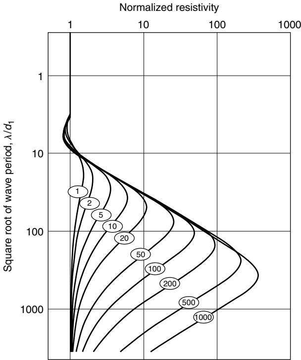
Figure 13.14 Magnetotelluric sounding curves for a three-layer sequence. The middle layer is a virtual insulator, while the first and last layers have a common resistivity. The ratio of the thickness of the second layer to that of the first is indicated by the label on each curve.
